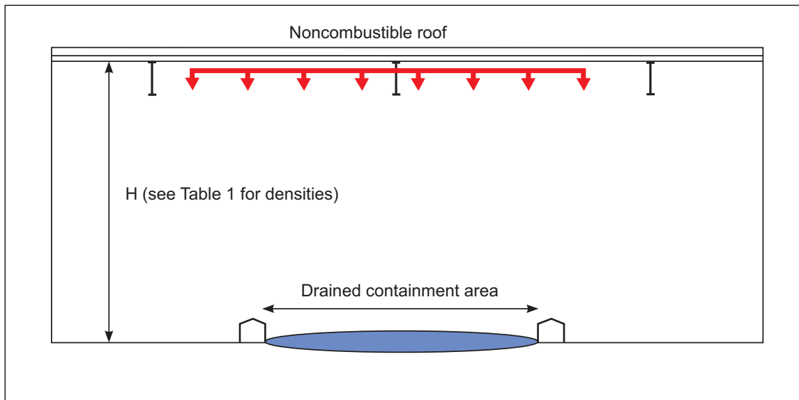
Fig. 2.4.4.2.2(A). Roof level sprinkler option
