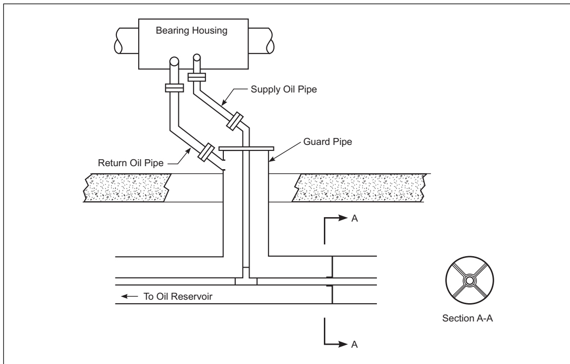
Fig. 2.2.7.1 Guard piping
