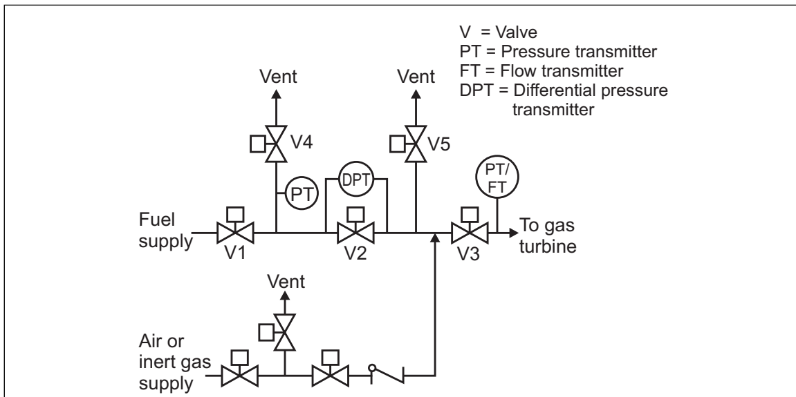
Fig. 2.5.2.1.2(B). Gaseous fuels (triple block, double vent, and pressurized pipe section)
