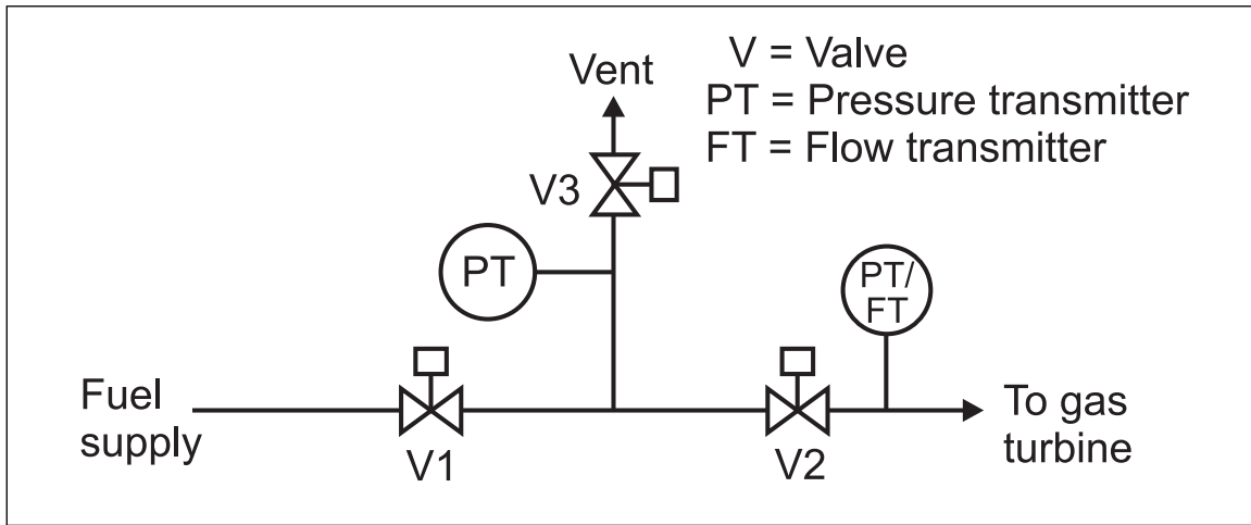
Fig. 2.5.2.1.1. Typical gaseous fuel system (double block and vent)
