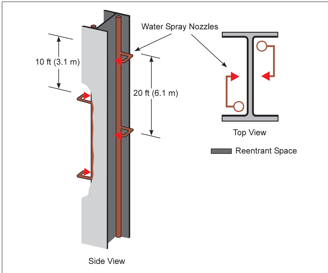
Fig. 2.2.3. Water spray protection for steel columns
