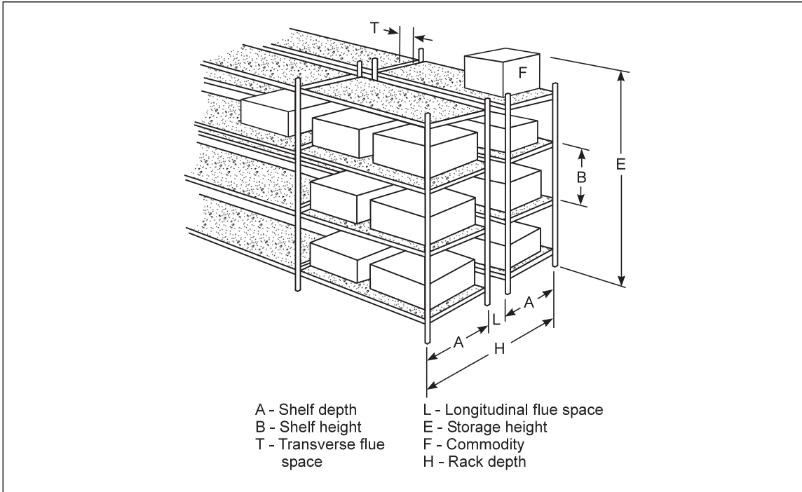
Fig. A-5. Double-row racks with solid shelves
