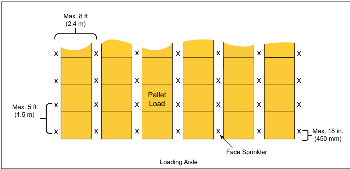
Fig. 14. Plan view of IRAS(E) horizontal in-rack sprinkler arrangement for multiple-row racks
