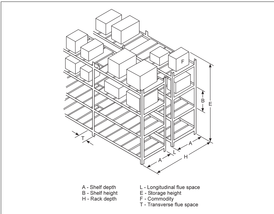
Fig. A-6. Double-row racks with slatted shelves
