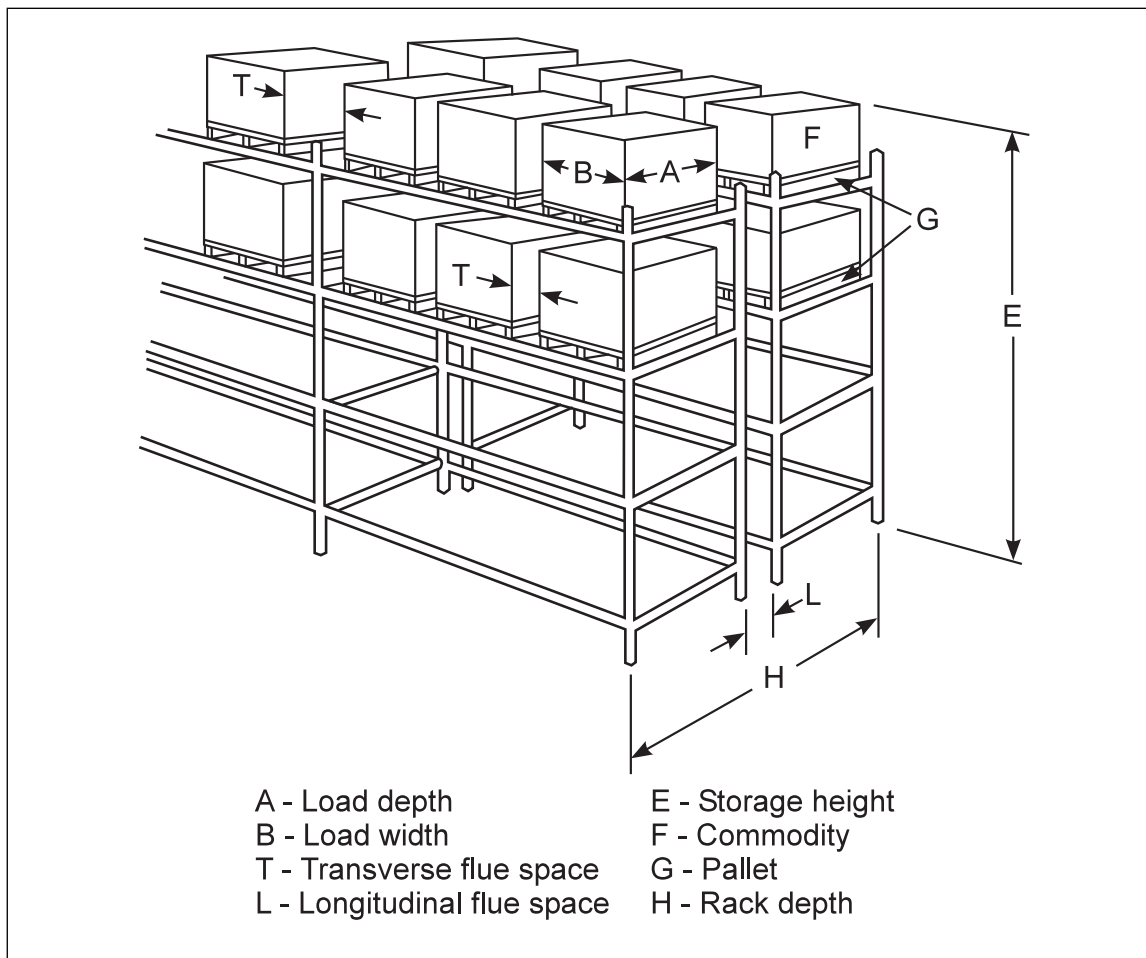
Fig. A-4. Open-frame double-row racks
