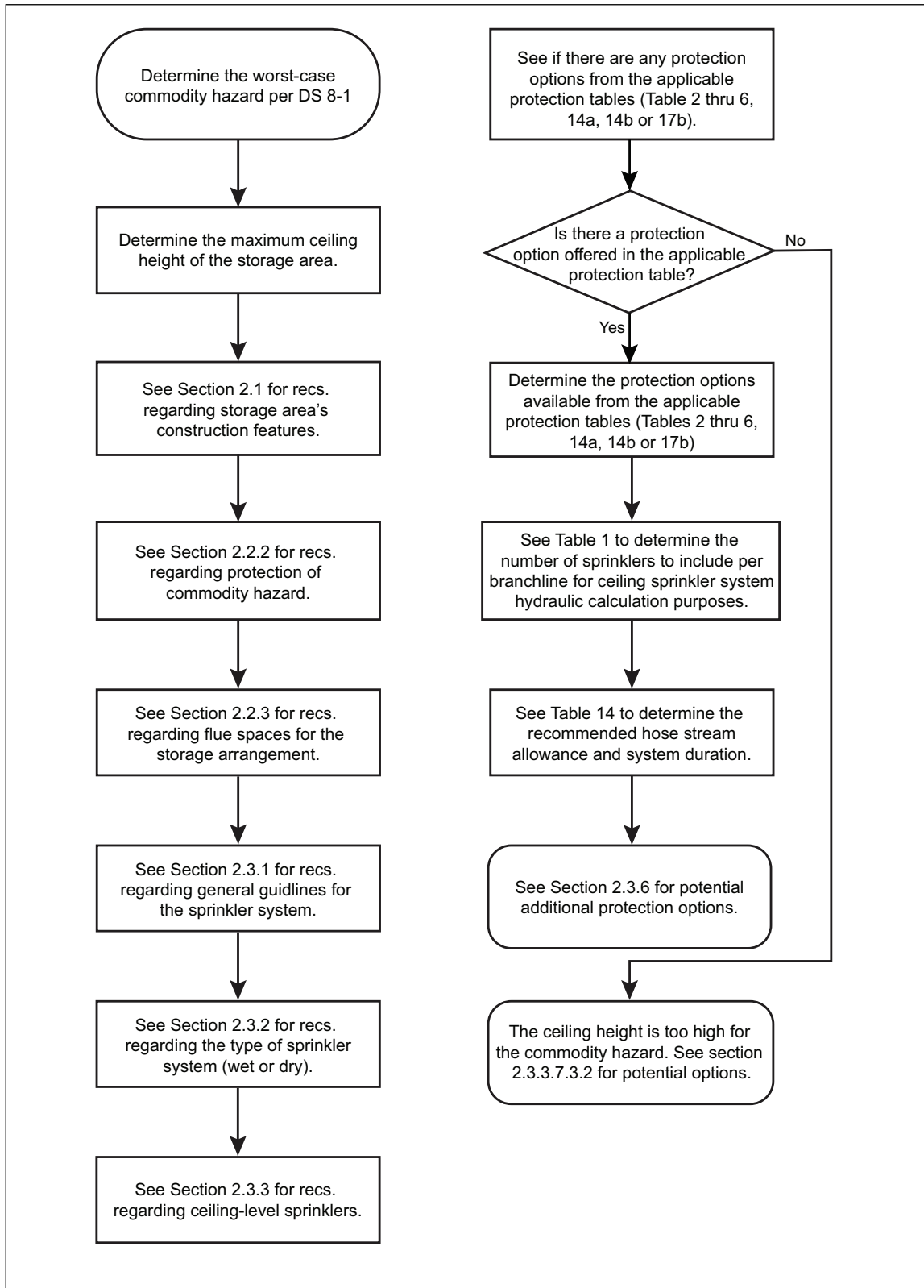
Fig. 1. Flowchart for determining the protection options for solid-piled, palletized, shelf, and bin-box storage arrangements
