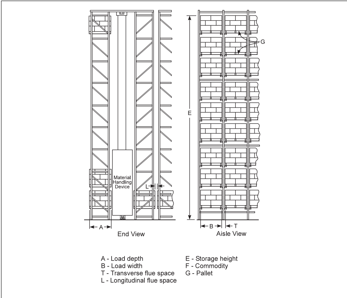
Fig. A-7. Automatic storage rack
