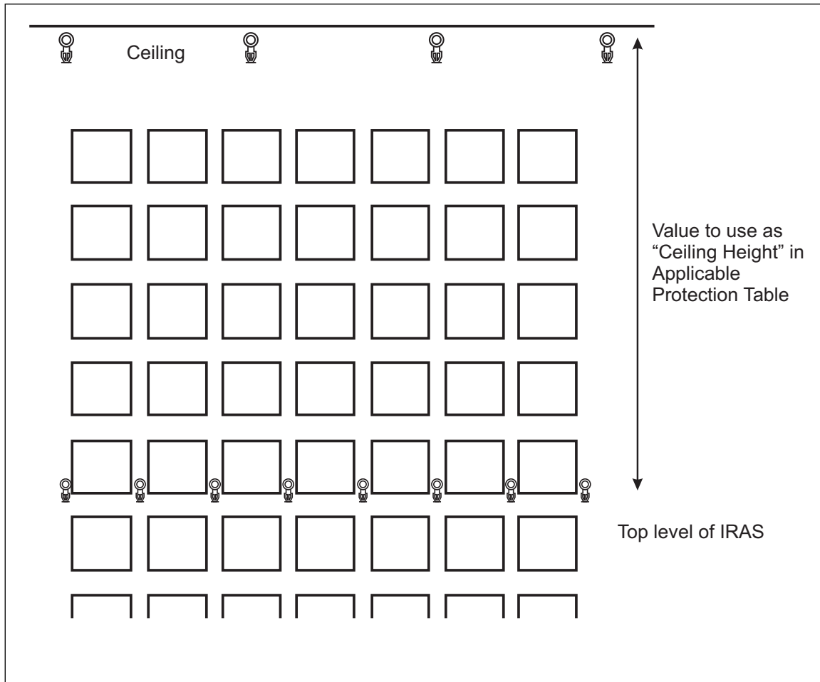
Fig. 22. Determining ceiling height in applicable protection table
