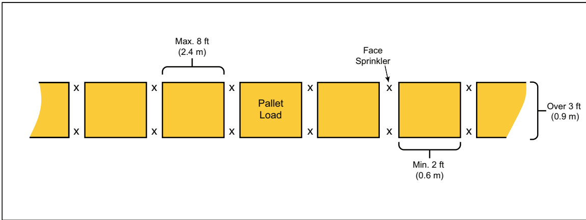
Fig. 11a. Plan view of IRAS(E) horizontal in-rack sprinkler arrangement for single-row racks over 3 ft (0.9 m) wide
