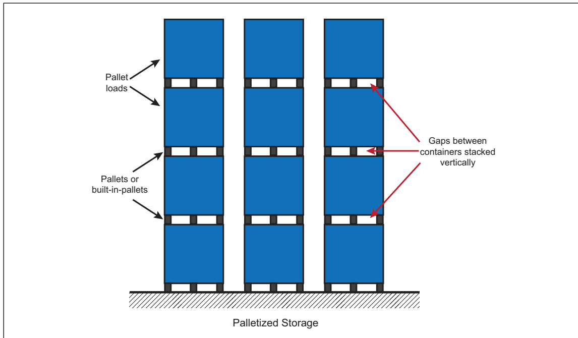
Fig. A-2. Example of a palletized storage arrangement
