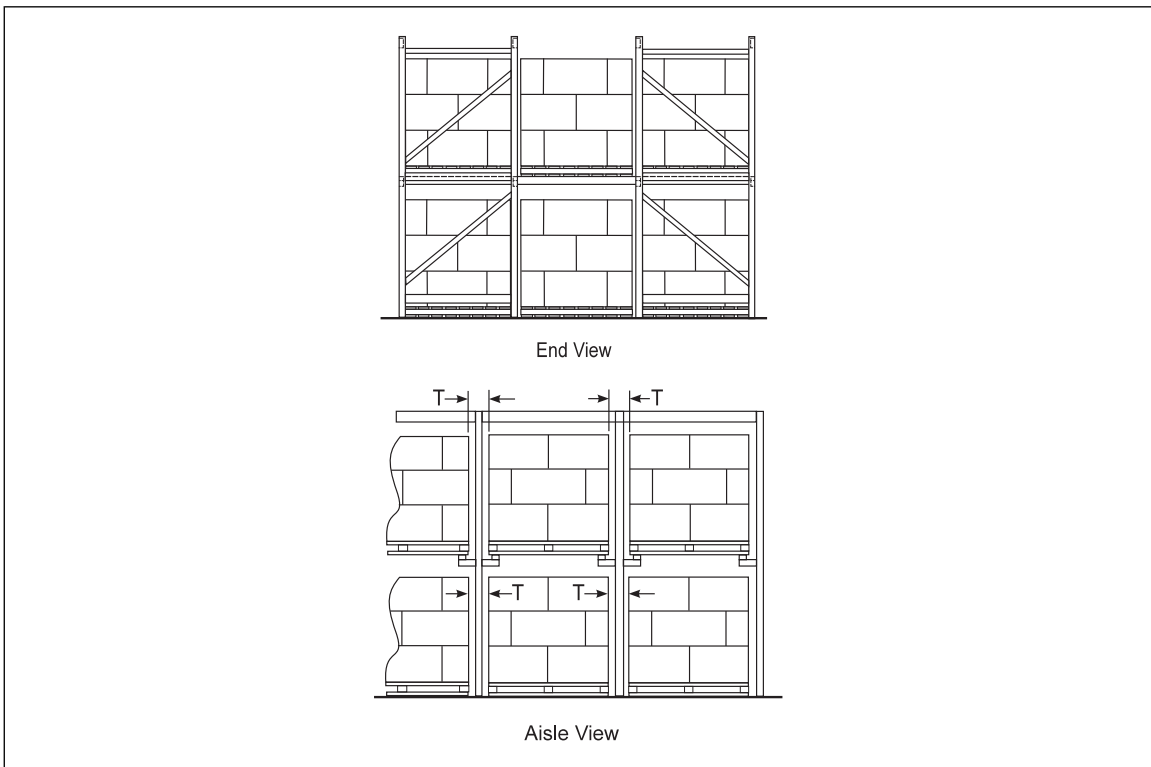
Fig. A-10. Drive-in rack, two or more pallets deep
