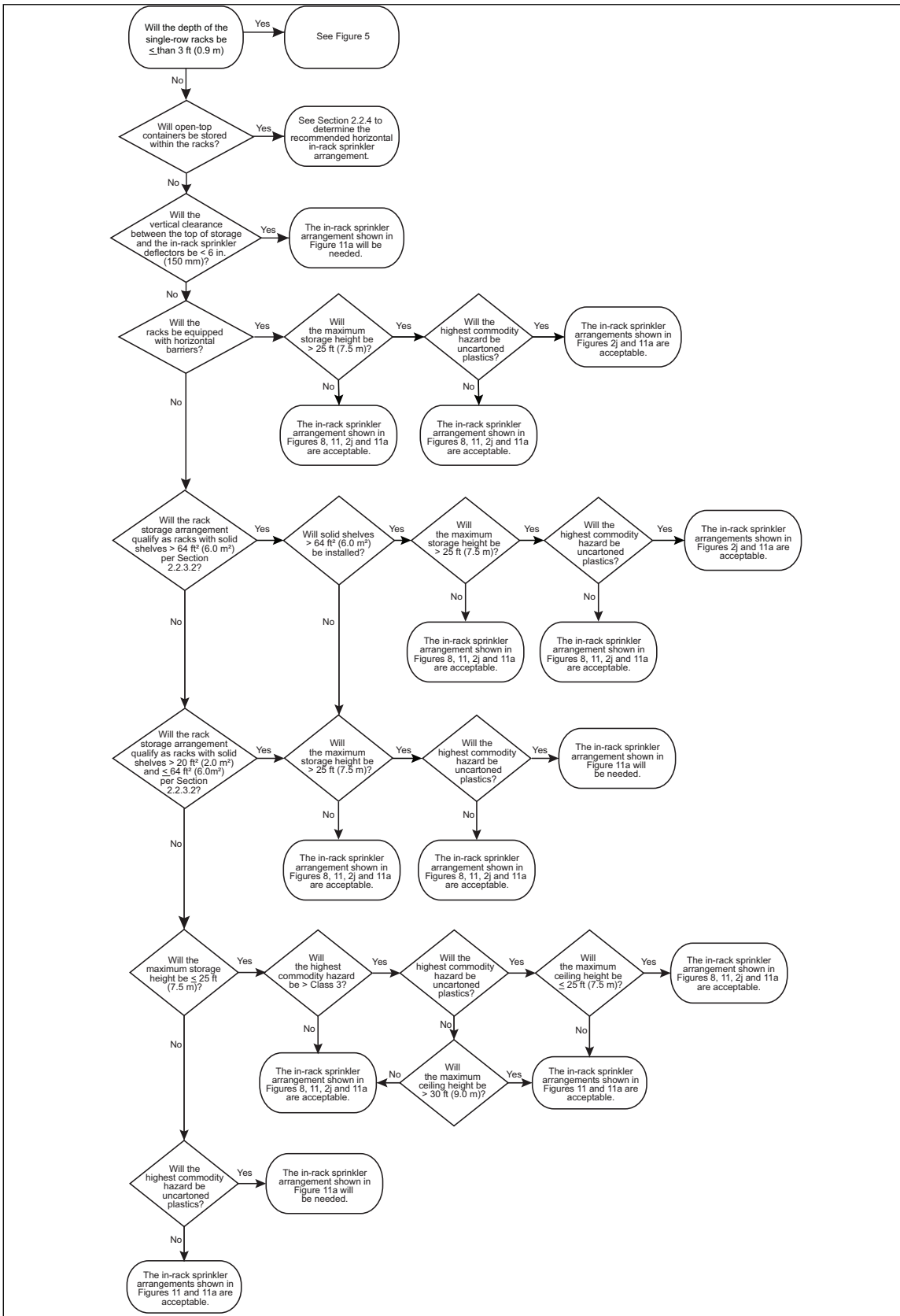
Fig. 5a. Recommended horizontal in-rack sprinkler arrangements for single-row racks over 3 ft (0.9 m) deep
