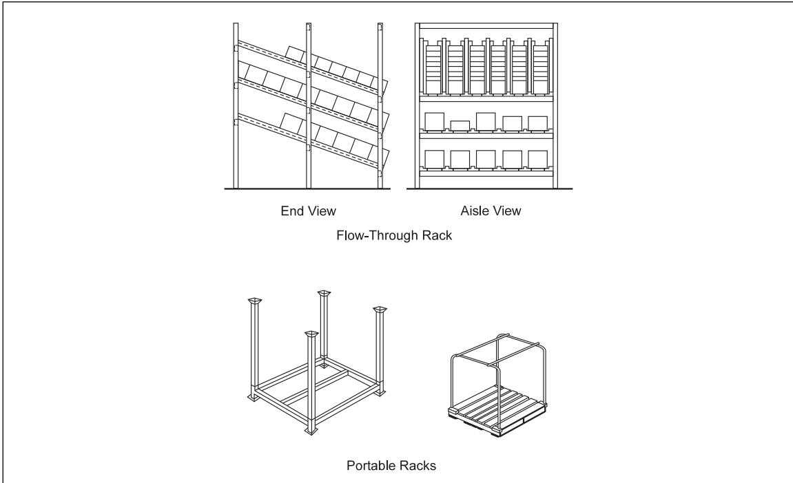
Fig. A-11. Flow-through and portable racks
