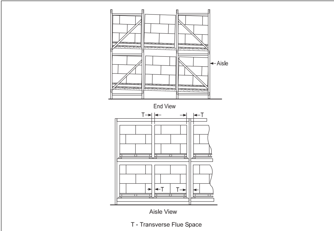
Fig. A-9. Flow-through pallet rack
