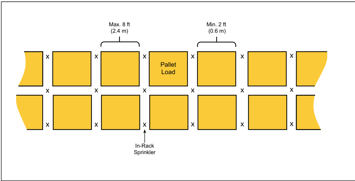
Fig. 13. Plan view of IRAS(E) horizontal in-rack sprinkler arrangement for double-row racks (face and flue)
