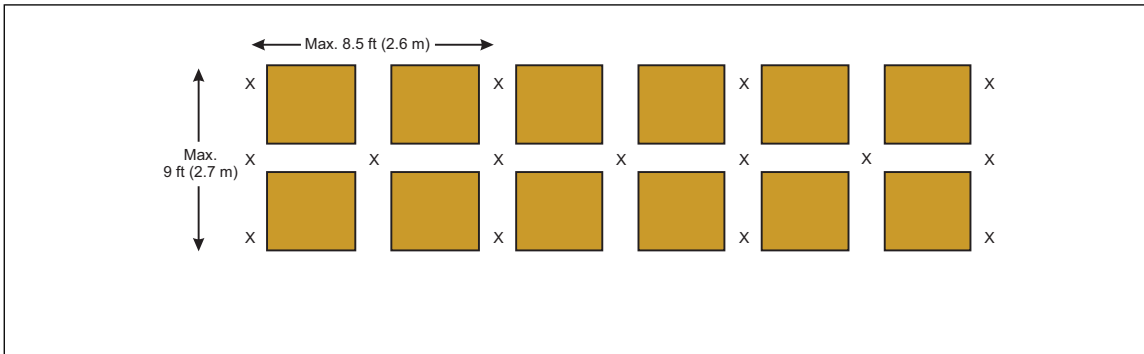
Fig. 20a. Plan view of alternative in-rack sprinkler arrangement for double-row racks up to 9 ft (2.7 m) deep
