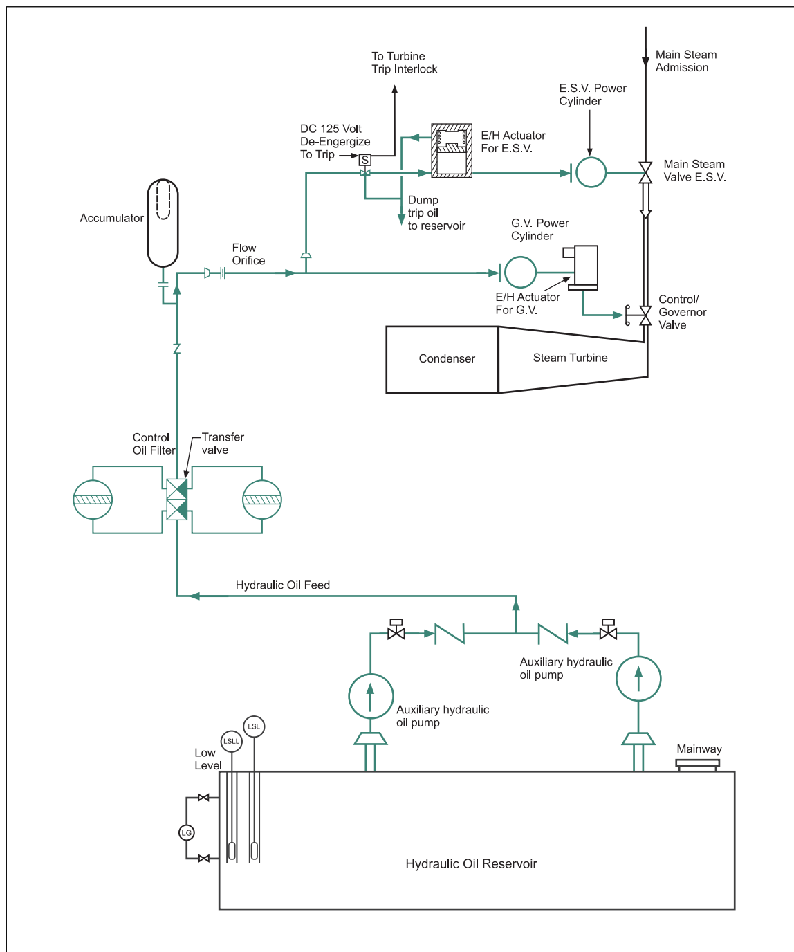
Fig. 2.1.5.1. Typical hydraulic control-oil supply system
