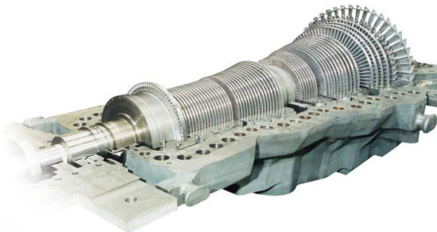
Fig. C.2-2. Generator-drive steam turbines at industrial facilities - rotor assembly with lower case (General Electric Company, all rights reserved, used with permission)
