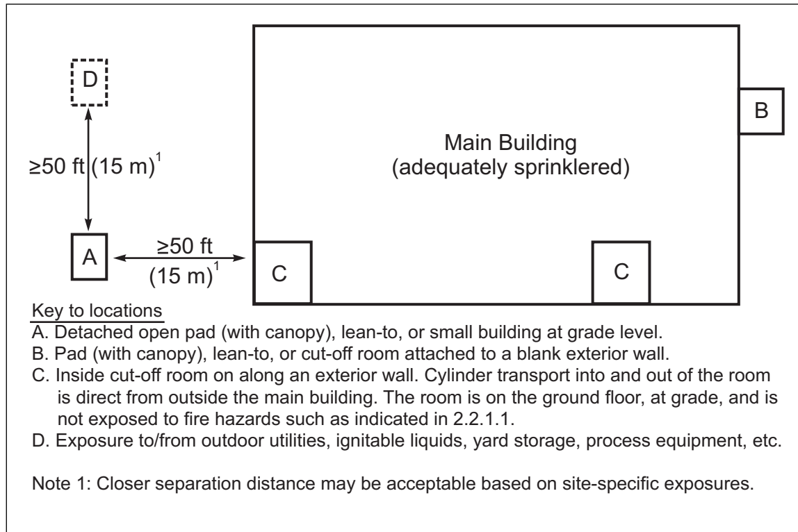
Fig. 1. Cylinder storage and dispensing locations
