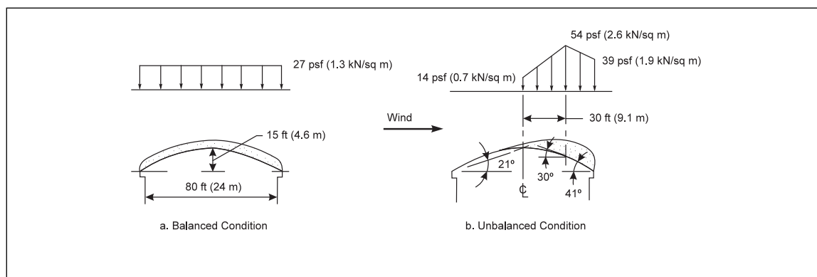
Fig. F.1-2B. Design snow loads for Example 2 using the Data Sheet recommendations of Appendix C
