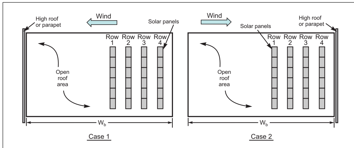
Fig. 2.5.2.3-8. W_b for snow drift at parapets, roof projections, or high roof walls for flush-mounted solar panels, widely-spaced tilted solar panels, and tilted solar panels with less than significant height
