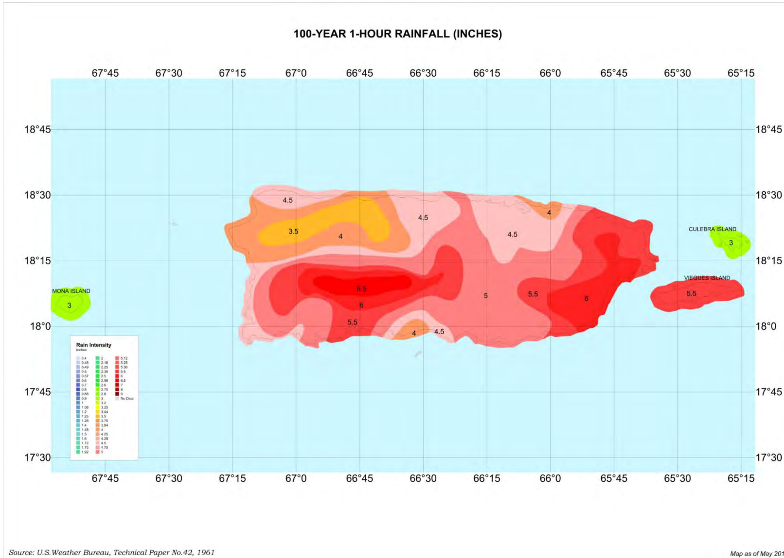
Fig. D7. Rainfall intensity (i) in inches per hour for Puerto Rico (to convert to millimeters per hour multiply by 25.4)
