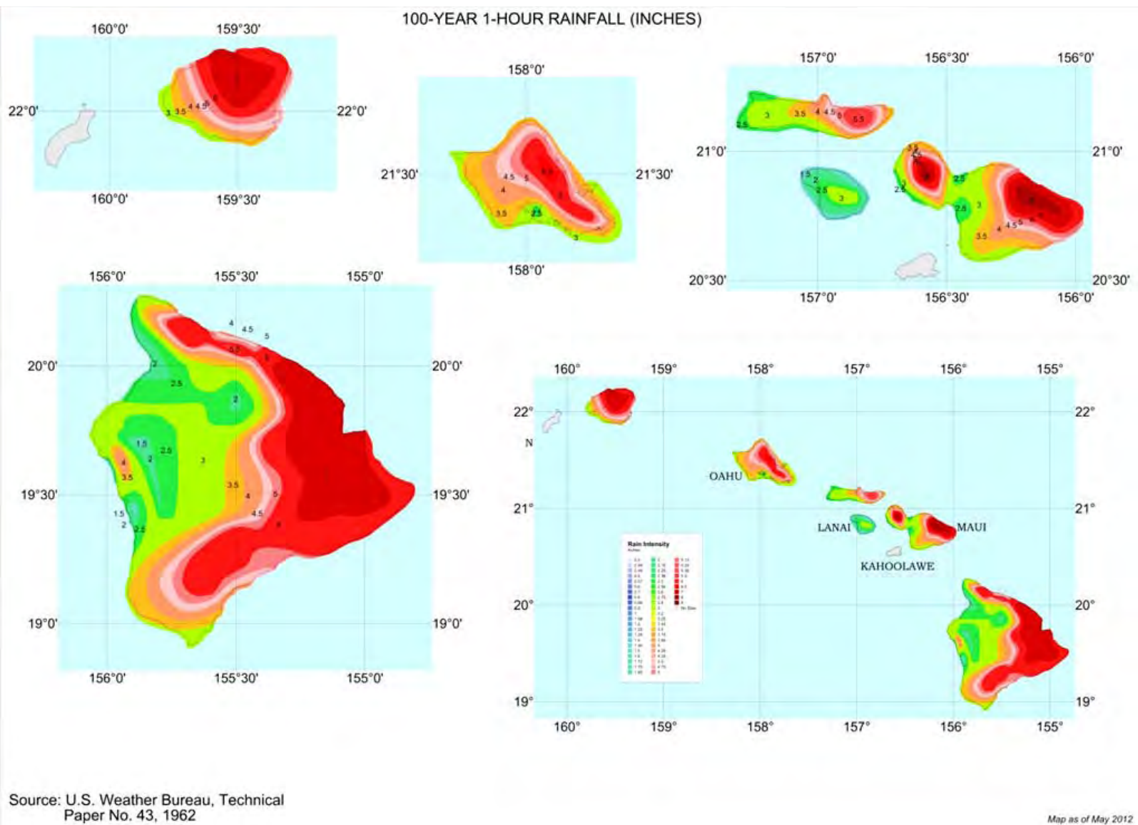
Fig. D8. 100-year, 60-minute Rainfall intensity ( i ) in inches per hour for Hawaiian Islands (to convert to millimeters per hour multiply by 25.4)
