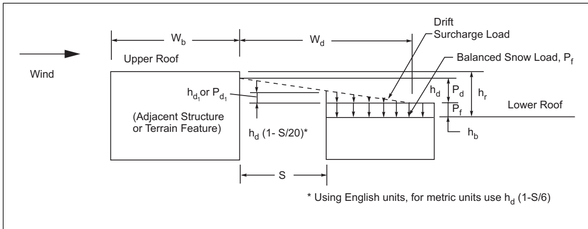
Fig. C.3.1.2-8. Snow loads for lower roof of adjacent structures
