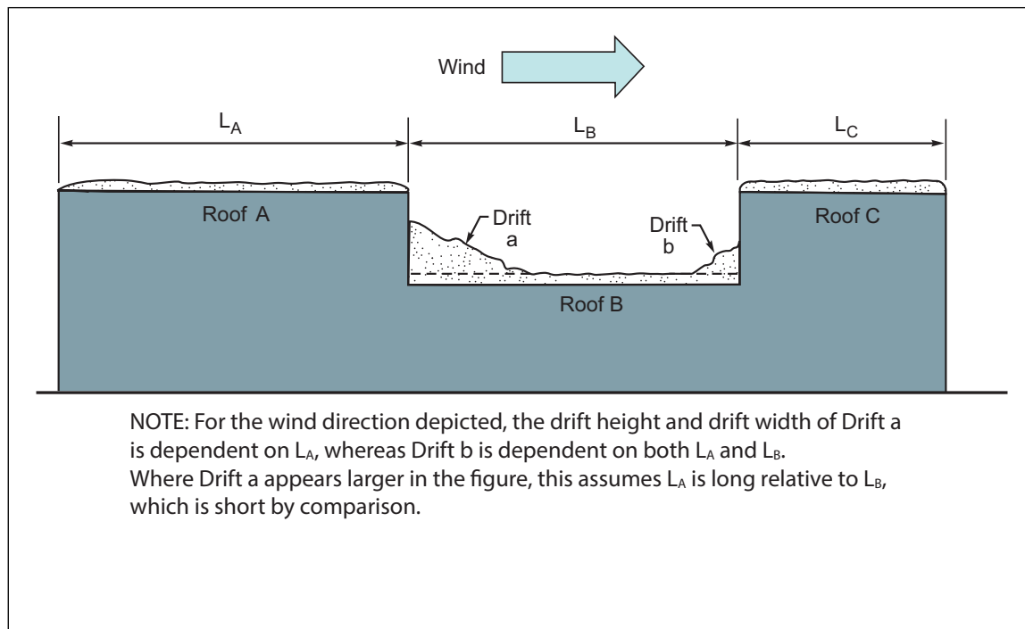
Fig. C.3.1.2-6. Windward and leeward drifting at a roof pocket
