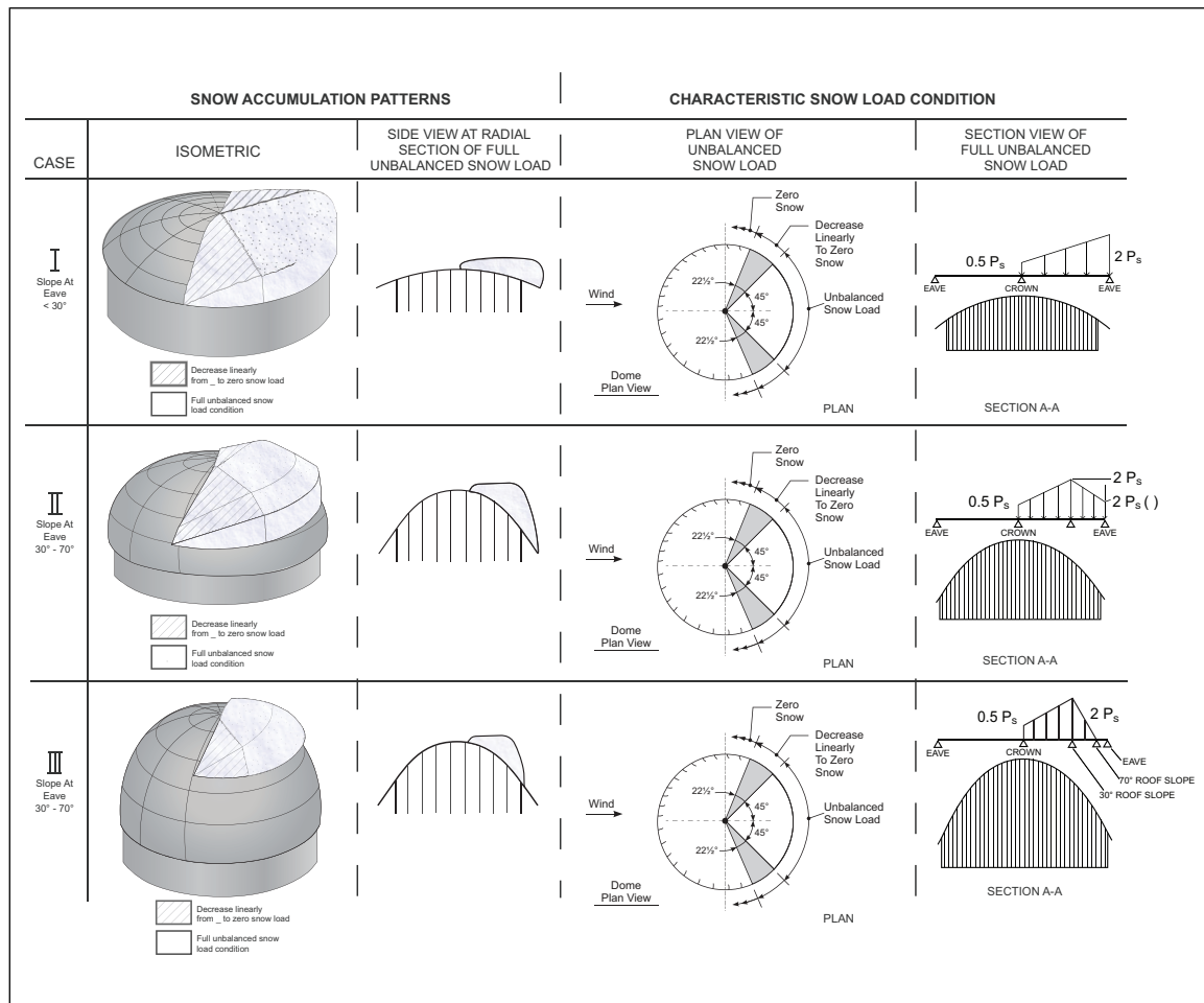
Fig. C.3.1.2-2. Unbalanced snow load distribution on dome roofs
