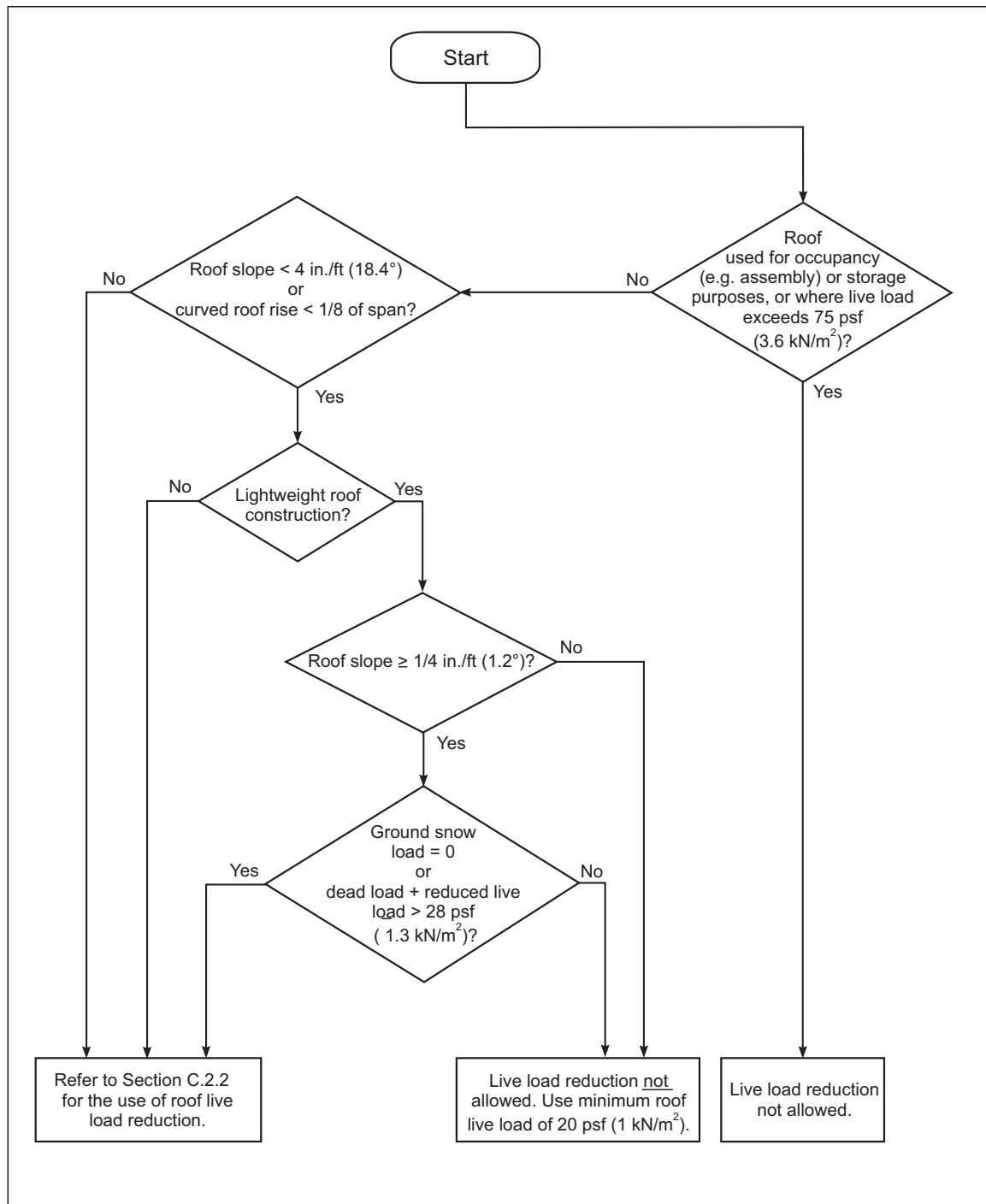
Fig. C.2.1. Roof live load reduction flow chart
