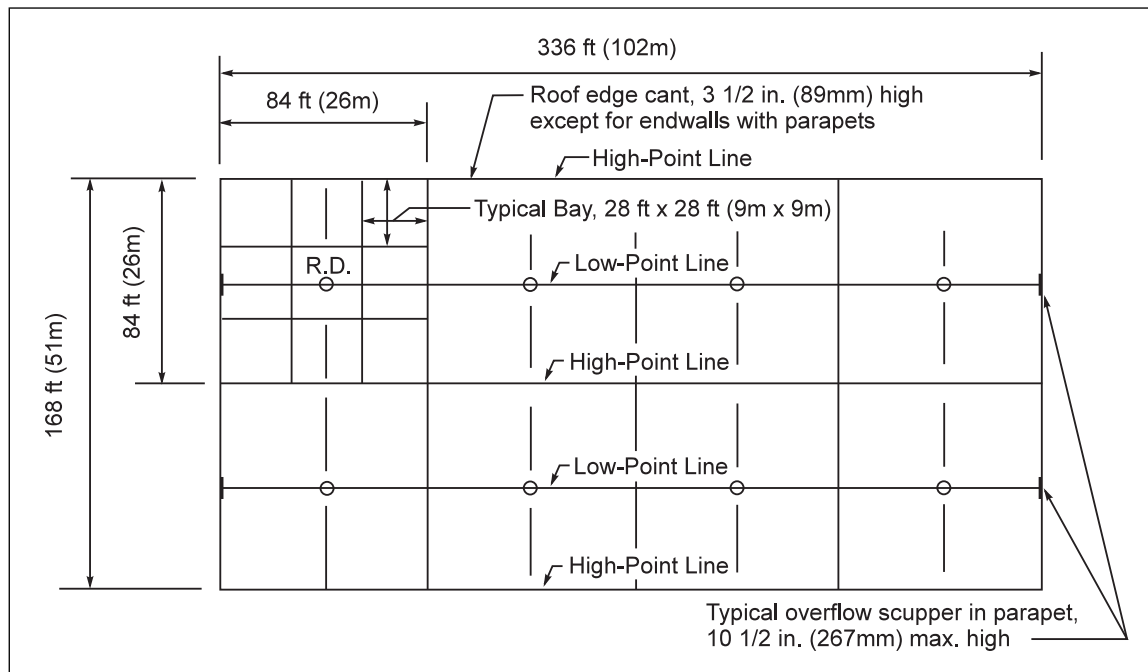
Fig. F.2-1. Sloped roof plan for Example 5
