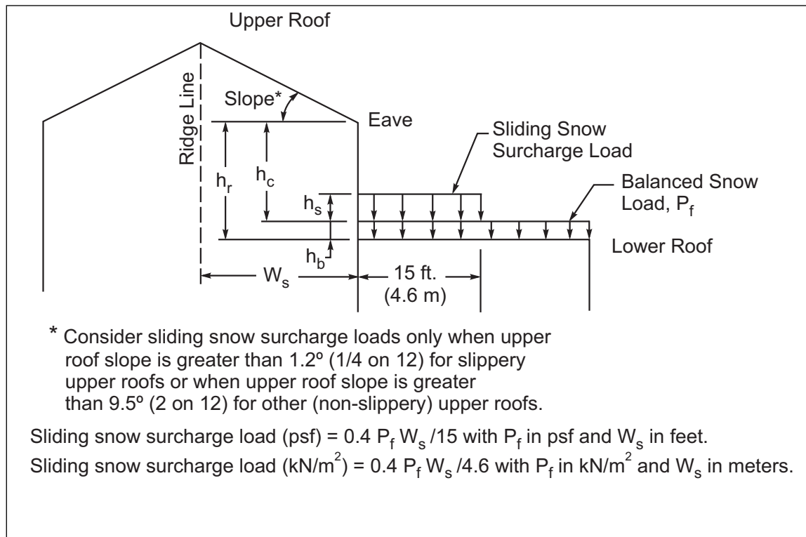
Fig. C.3.1.2-10. Sliding snow for lower roofs (upper roof snow load not shown)
