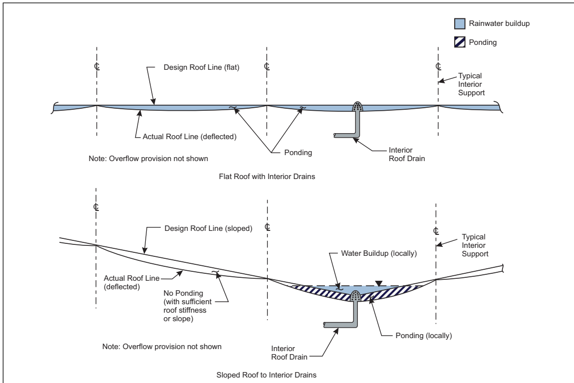
Fig. 2.4.4.1-3. Flat and sloped roofs with interior roof drains
