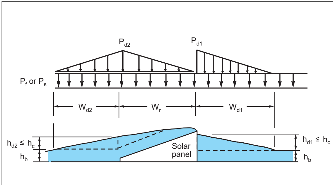
Fig. 2.5.2.3-9. Snow drift loads at tilted closed-back solar panel widely spaced rows (or a single row)
