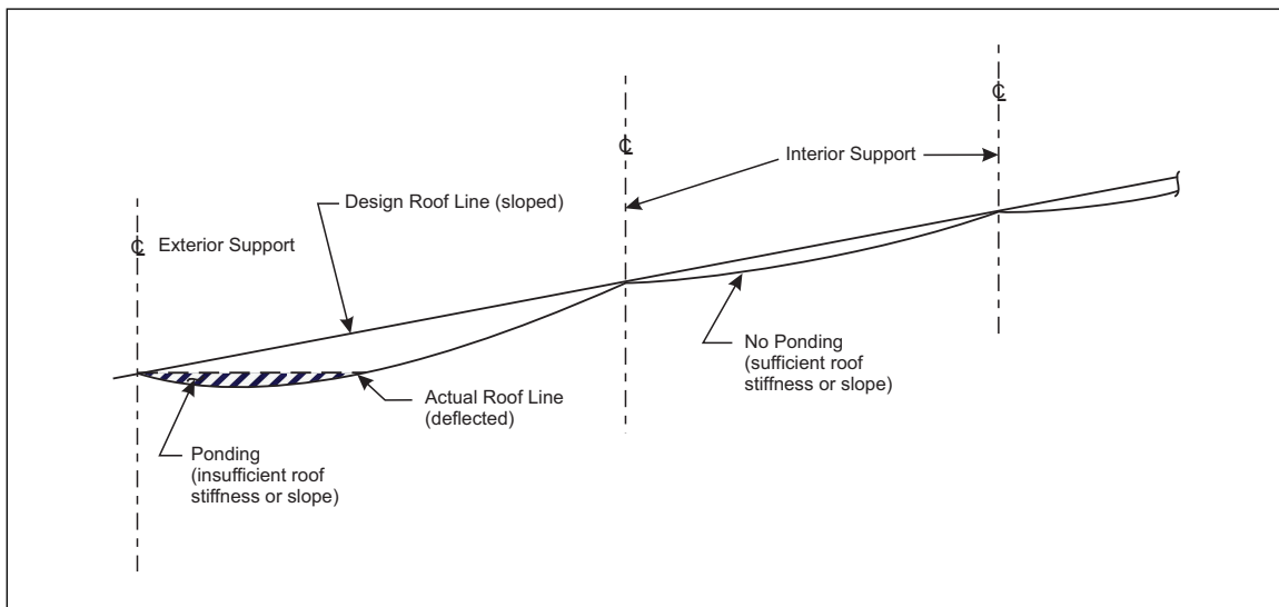
Fig. 2.4.4.1-4. Sloped roof with roof edge drainage
