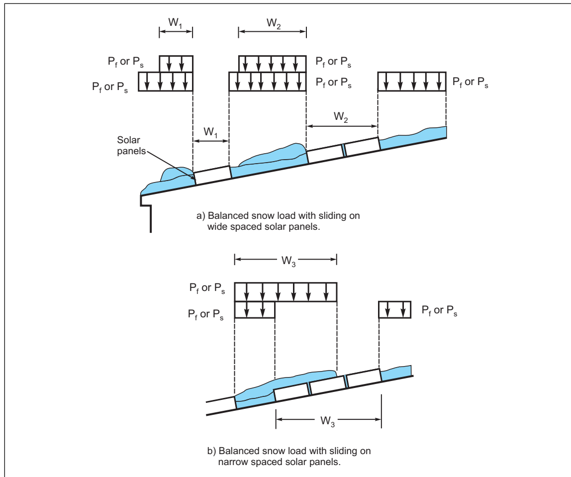
Fig. 2.5.2.3-16. Balanced snow plus sliding snow load with flush-mounted solar panels
