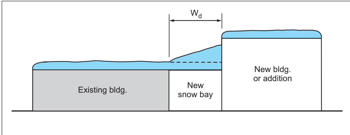
Fig. 2.3.4. New snow bay to prevent drift loading on an existing roof
