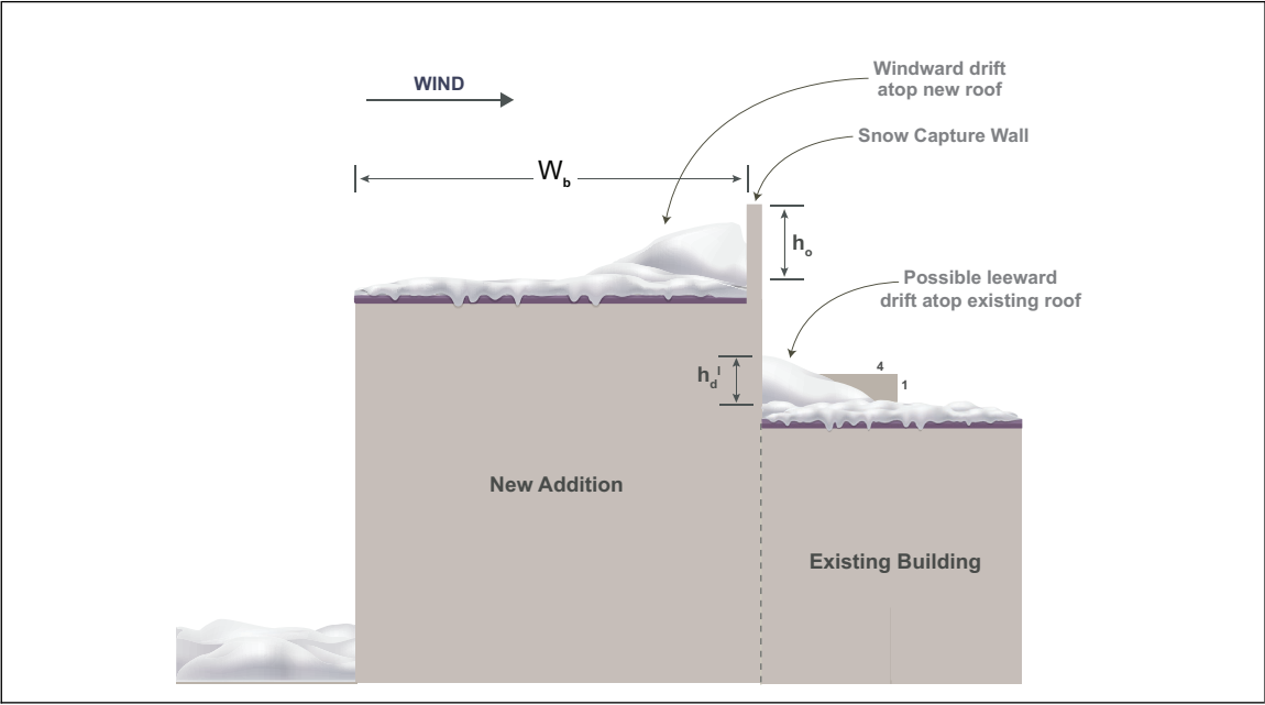
Fig. 2.3.3.2 Snow capture wall
