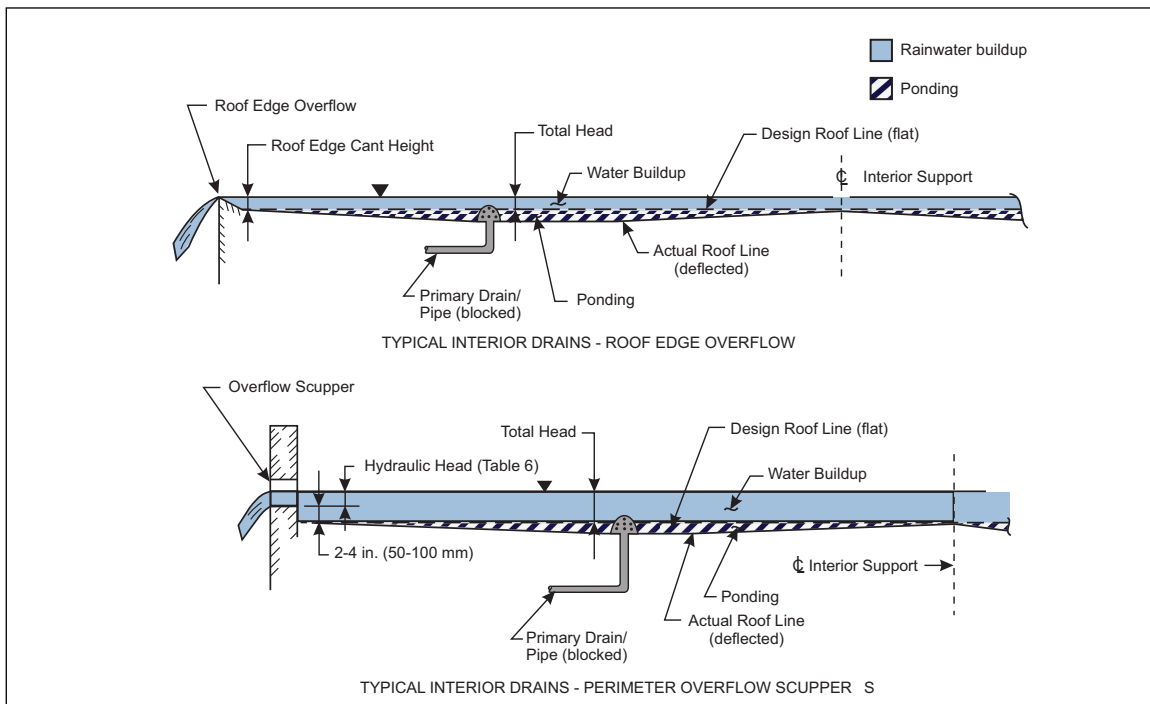
Fig. 2.4.2.1-2. Typical primary and overflow drainage systems for flat roofs
