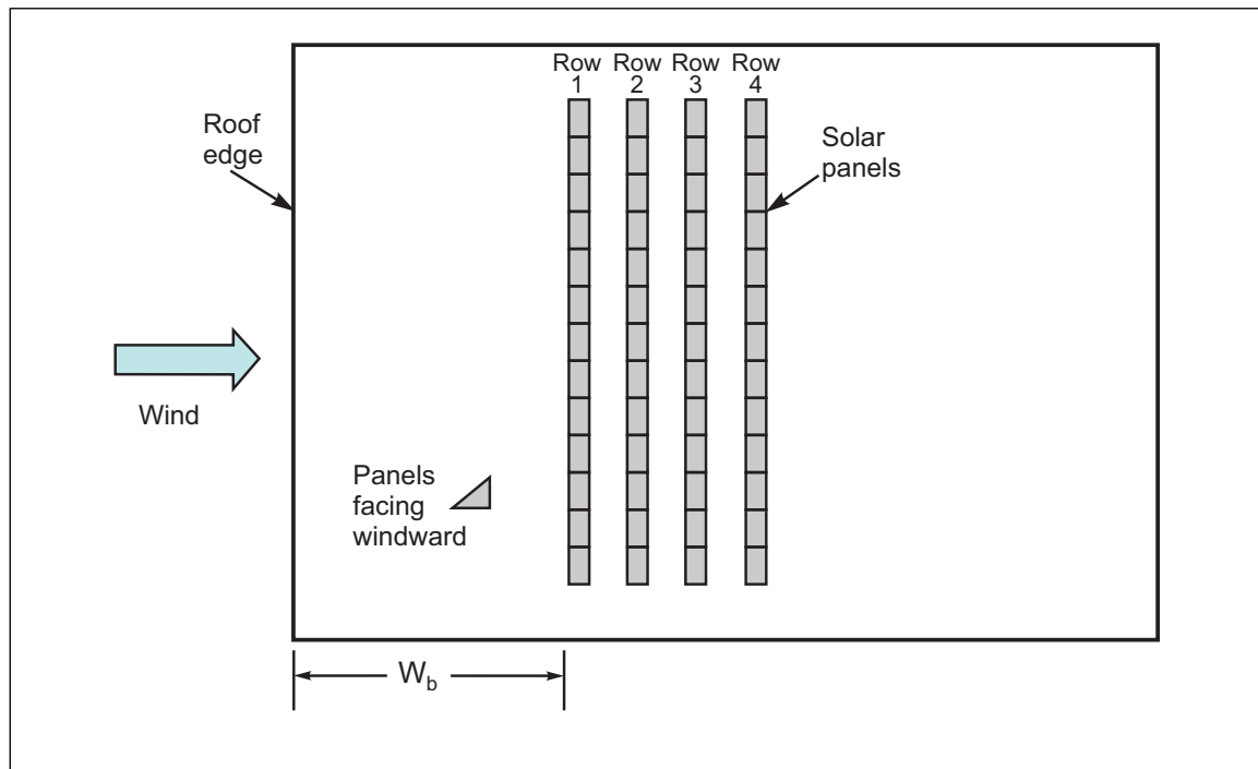
Fig. 2.5.2.3-12. Upwind fetch distance ( W_b ) for snow drift at multiple rows of closely spaced tilted solar panels with panels facing windward
