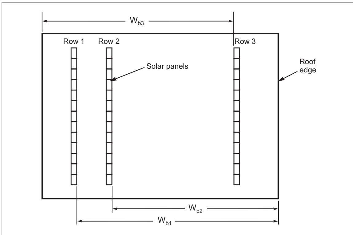
Fig. 2.5.2.3-10. Upwind fetch ( W_b ) for drift load at widely spaced, or single row, solar panels (drifting is not shown)
