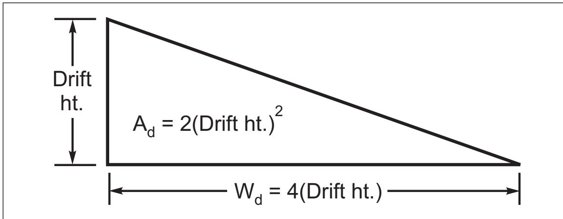
Fig. F.3-3. Unrestricted drift
