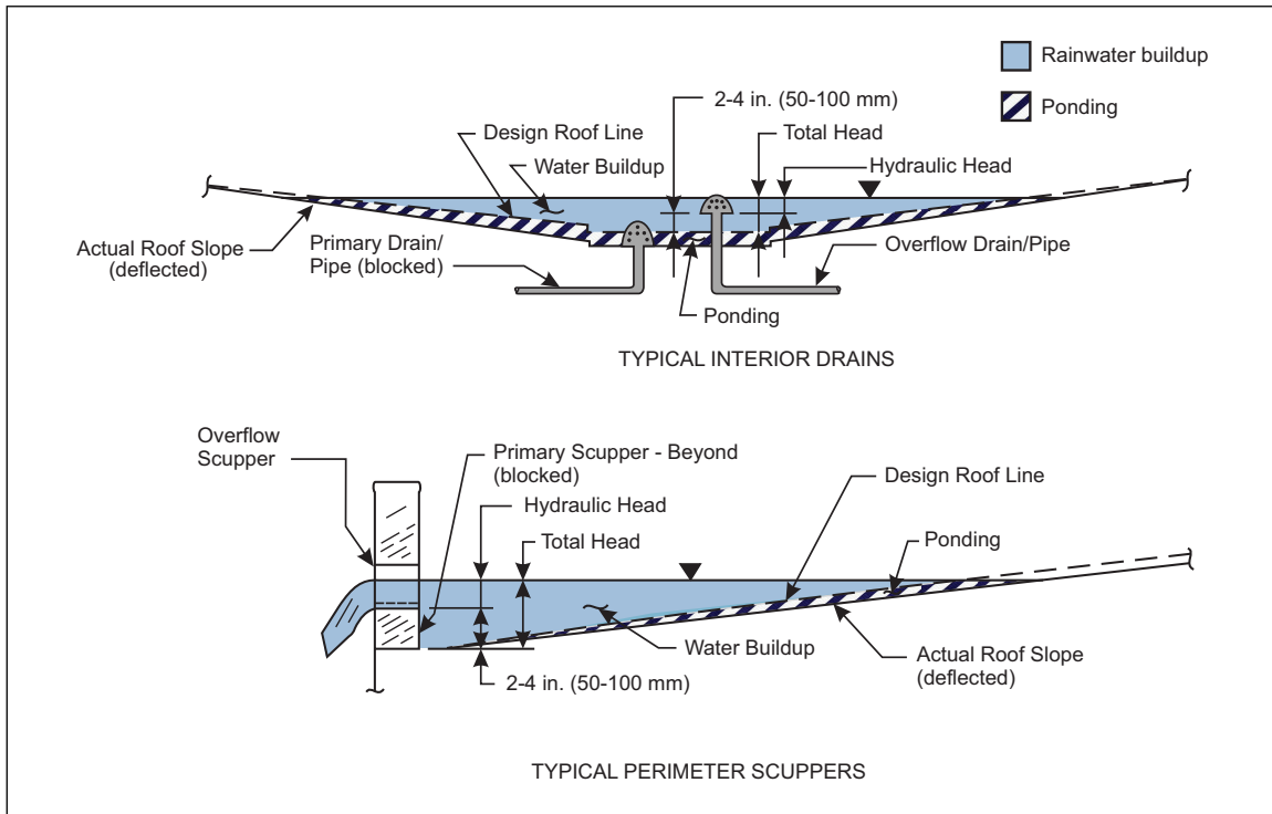
Fig. 2.4.2.1-1. Typical primary and overflow systems for pitched roofs
