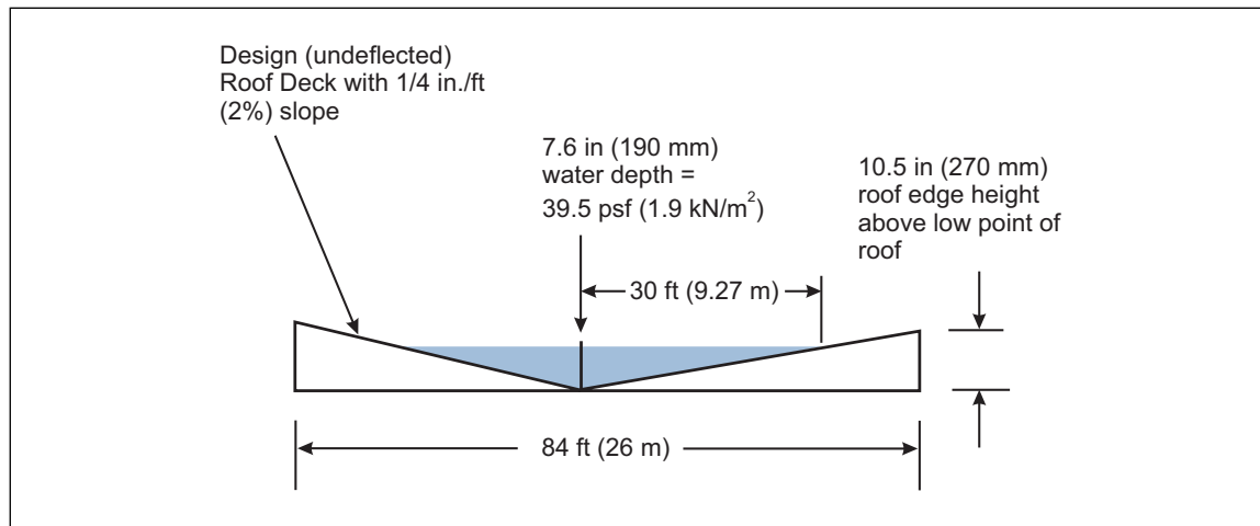
Fig. F.2-2. Sloped roof section for Example 5
