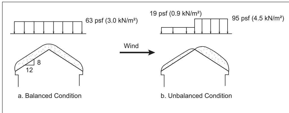
Fig. F.1-1. Design snow loads for Example 1
