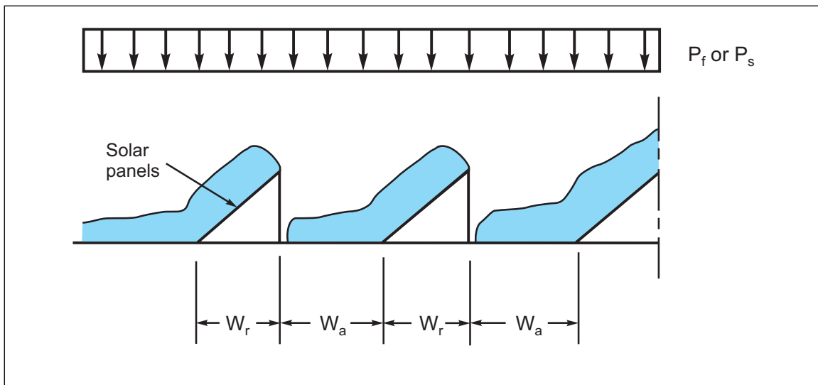
Fig. 2.5.2.3-4. Balanced snow loads on roofs with tilted solar panels
