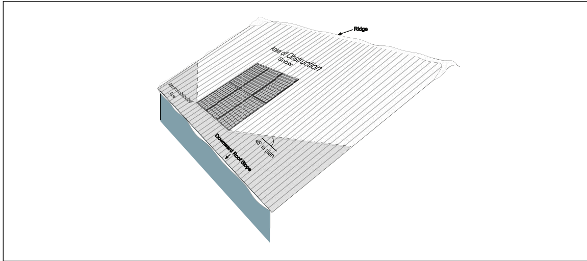
Fig. 2.5.2.3-2. Obstructed portions of sloped roofs
