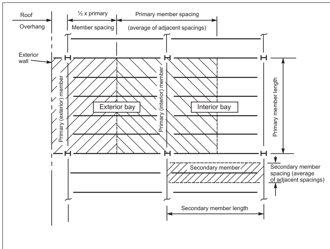
Fig. A.1.5. Typical tributary loaded areas
