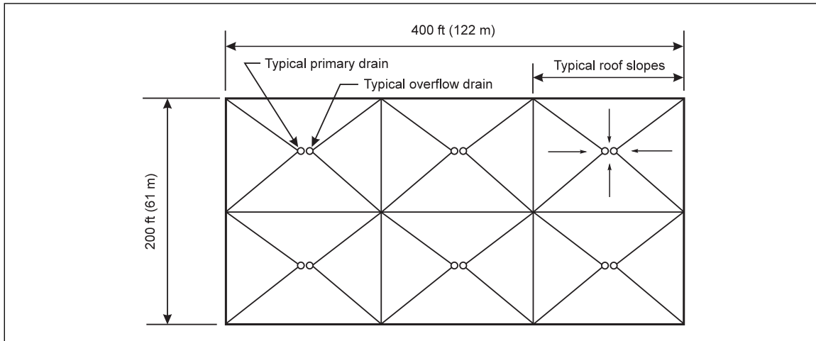
Fig. F.2-3. Roof plan for Example 6
