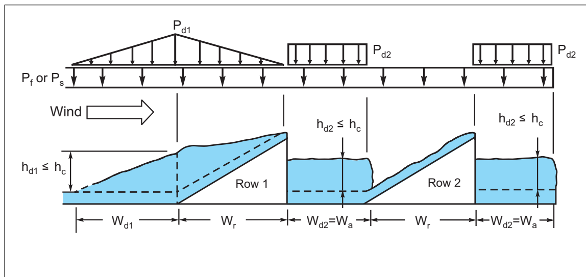
Fig. 2.5.2.3-11. Snow drift loads at tilted solar panels for closely spaced rows with panels facing windward
