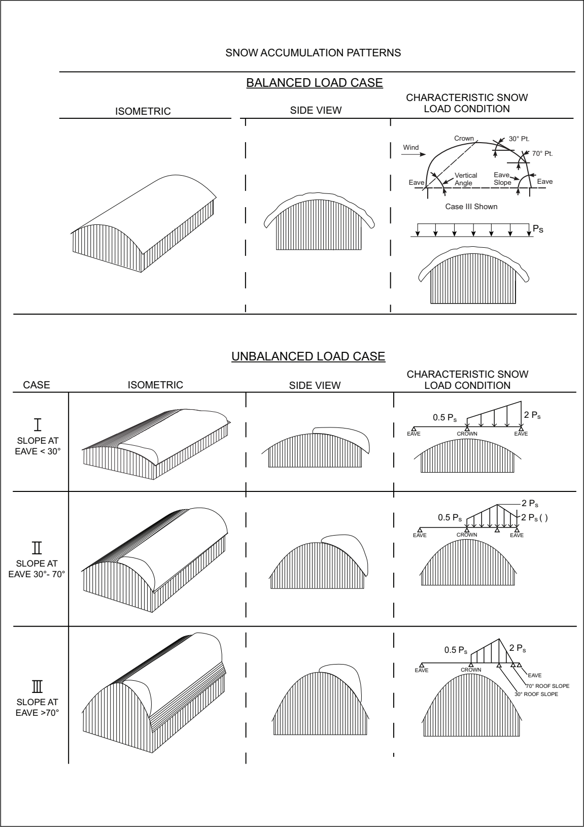
Fig. C.3.1.2-1. Snow loads for curved and dome roofs
