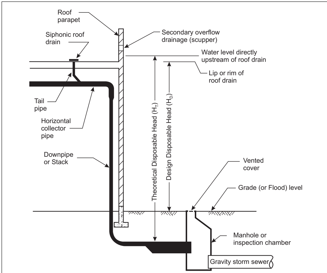
Fig. 2.4.4.2-2. Elevation view of siphonic system and disposable (available) head
