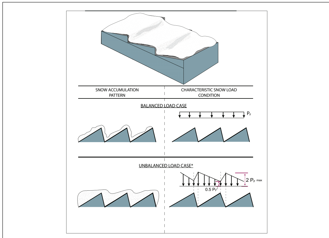
Fig. C.3.1.2-3. Snow loads for sawtooth valley roofs
