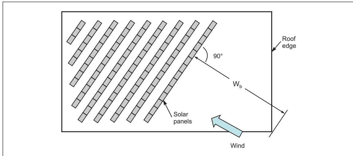
Fig. 2.5.2.3-15. Upwind fetch distance ( W_b ) for snow drift at closely spaced skewed rows of solar panels
