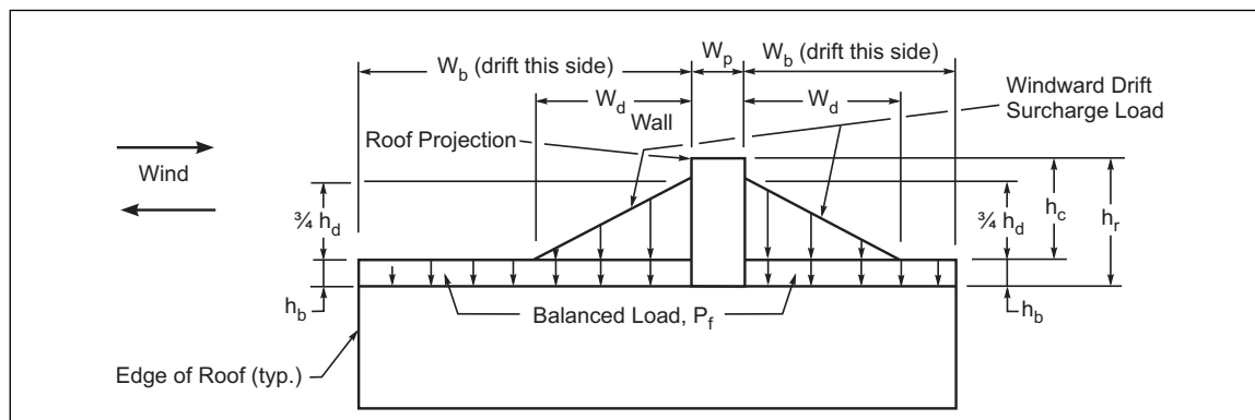
Fig. C.3.1.2-5. Snow load at roof projections
