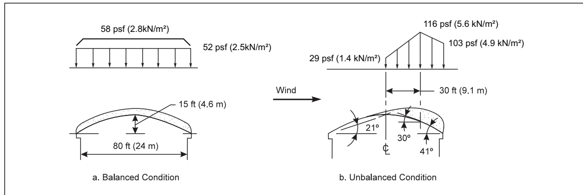
Fig. F.1-2A. Design snow loads for Example 2
