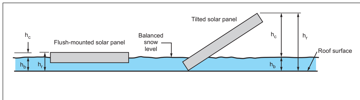
Fig. 2.5.2.3-1. Flush-mounted and tilted solar panels, schematic elevation view
