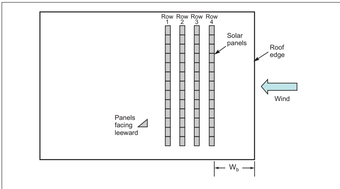
Fig. 2.5.2.3-14. Upwind fetch distance ( W_b ) for snow drift at multiple rows of closely spaced tilted solar panels with panels facing leeward
