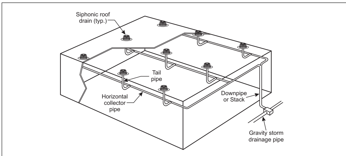
Fig. 2.4.4.2-1. Diagram of siphonic roof drain system
