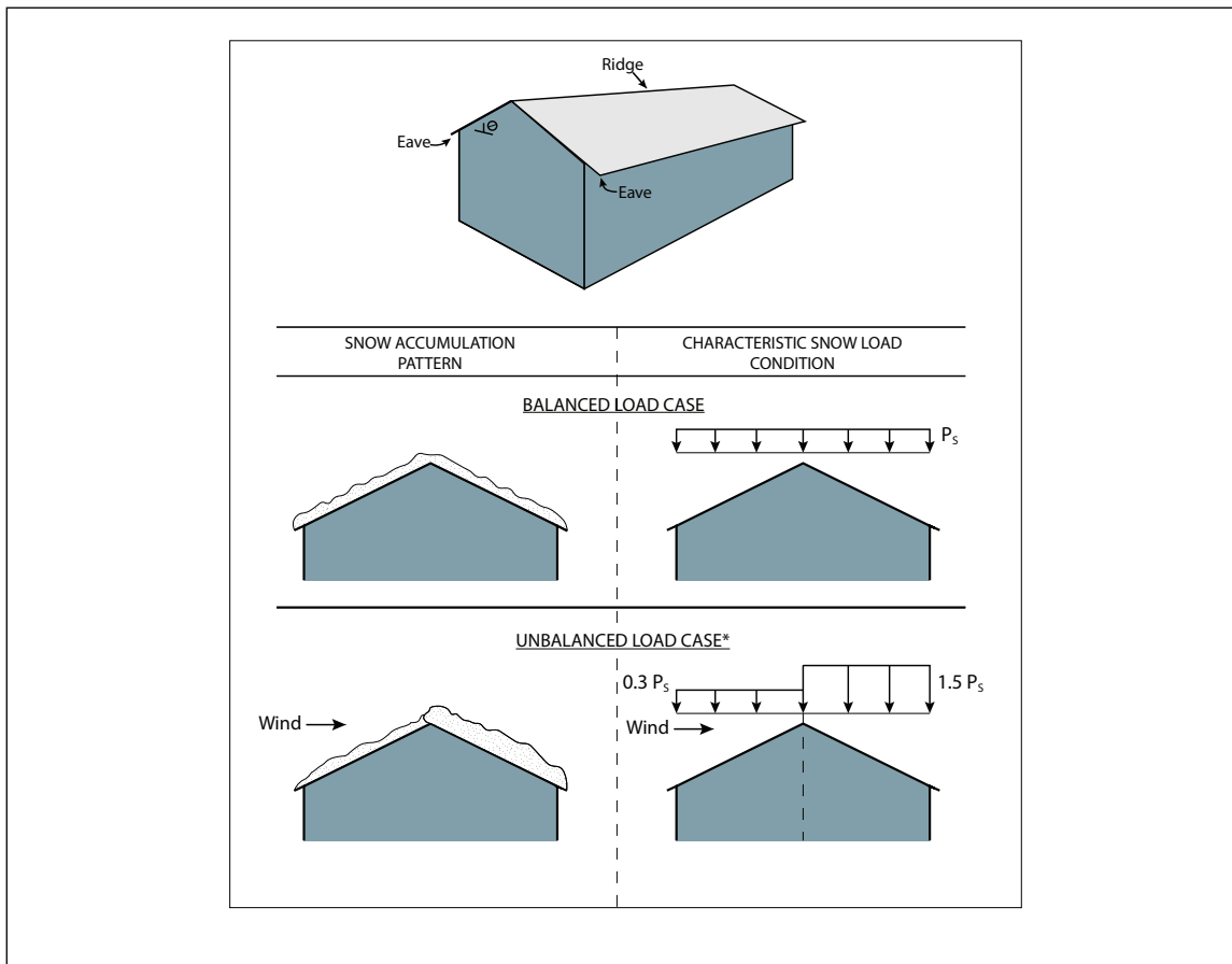
Fig. 2.2.1. Snow loads for hip and gable roofs
