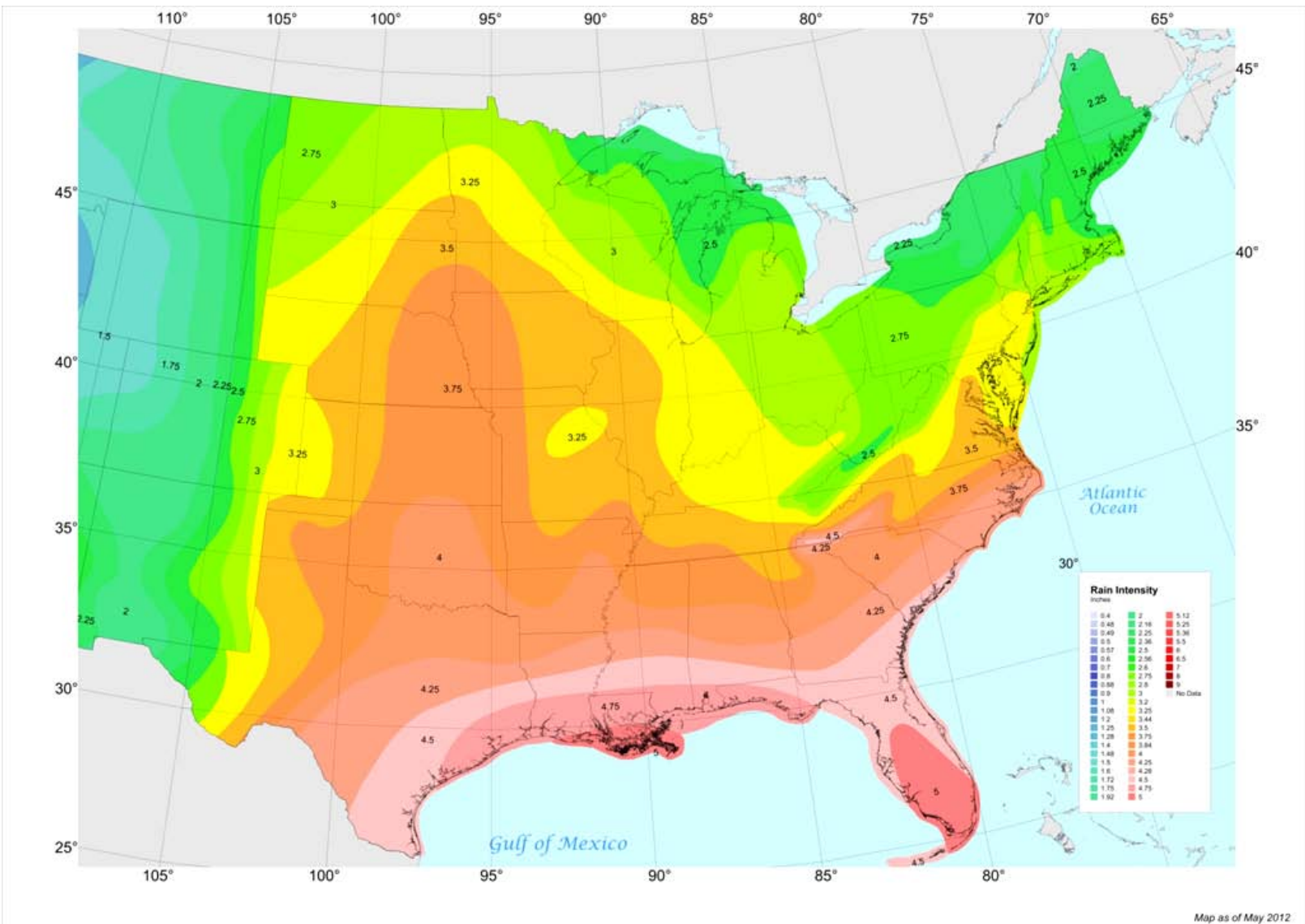
Fig. D6. 100-year, 60-minute Rainfall intensity (i) in inches per hour for the central and eastern United States (to convert to millimeters per hour multiply by 25.4)
