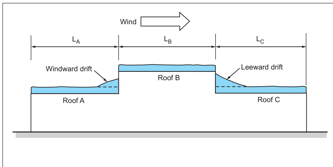
Fig. 3.3. Typical windward and leeward snow drifting
