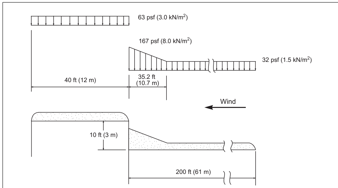
Fig. F.1-4. Design snow loads for Example 4A (Windward Drifting)
