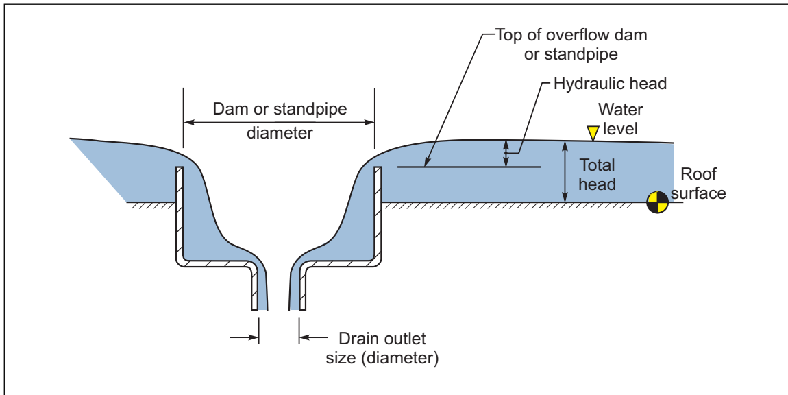
Fig. 2.4.4.1-2. Overflow (secondary) roof drain with hydraulic head and total head (debris guard not shown for clarity)
