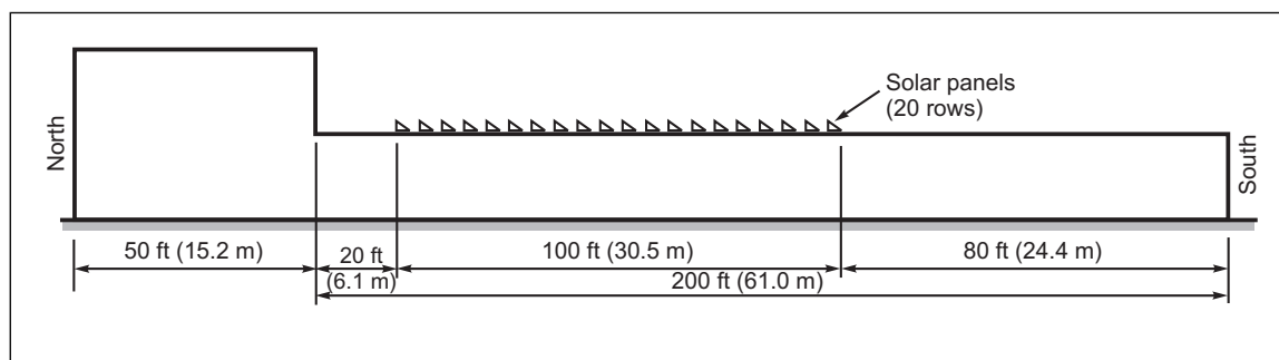
Fig. F.3-2. Elevation view of roof with solar panels
