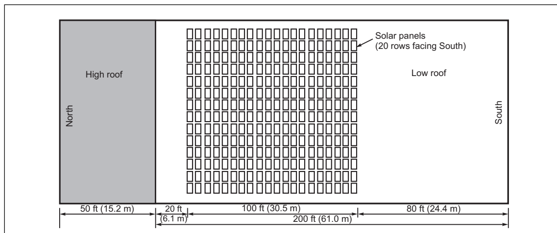
Fig. F.3-1. Plan View of Roof with solar panels
