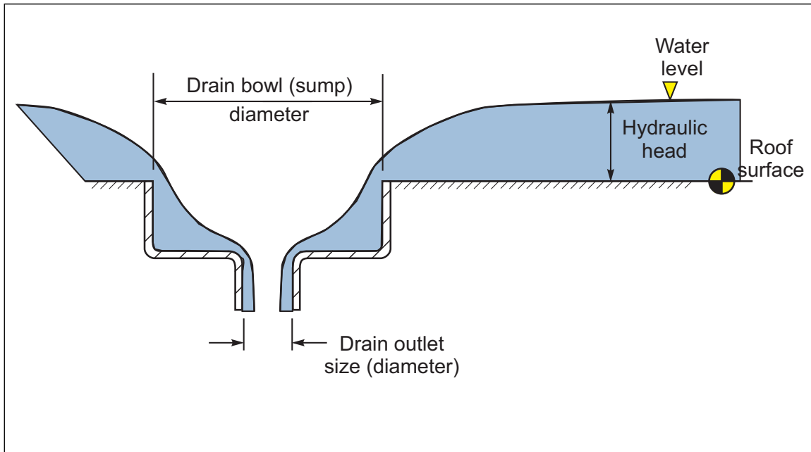
Fig. 2.4.4.1-1. Primary roof drain and hydraulic head (debris guard not shown for clarity)
