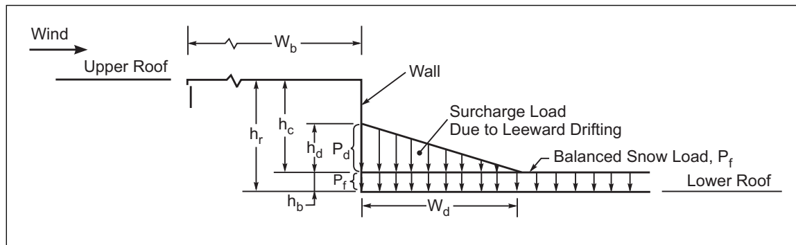
Fig. C.3.1.2-4. Leeward snow loads for lower roofs
