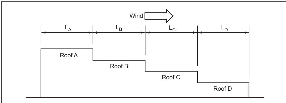
Fig. C.3.1.2-7. W_b for leeward snow drift at multiple roofs steps
