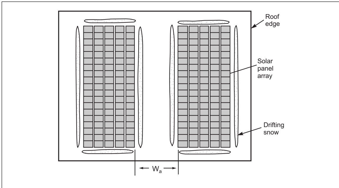
Fig. 2.5.2.3-7. Drifting snow load at flush-mounted solar panel arrays
