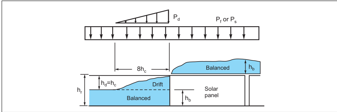
Fig. 2.5.2.3-6. Balanced and drifting snow load at flush-mounted solar panel array
