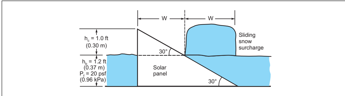
Fig. F.3-4. Sliding snow surcharge load at tilted solar panel
