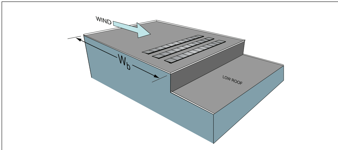
Fig. 2.5.2.3-5. Upwind fetch distance ( W_b ) for leeward snow drift at low roof with solar panels on high roof
