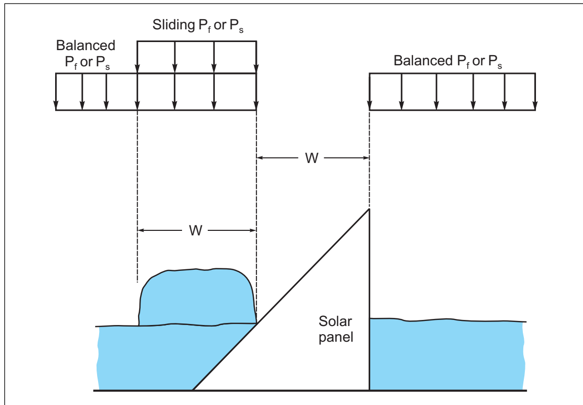
Fig. 2.5.2.3-17. Sliding snow load at tilted solar panels
