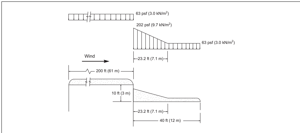
Fig. F.1-3. Design snow loads for Example 3A (Leeward Drifting)
