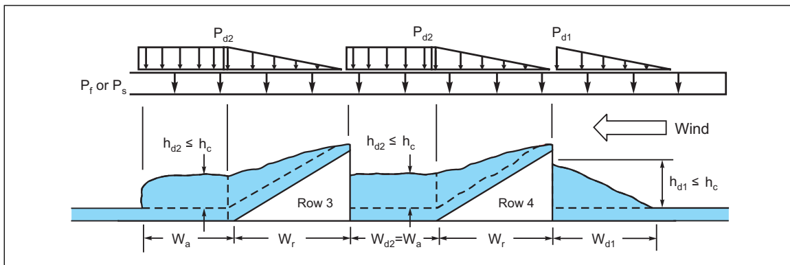
Fig. 2.5.2.3-13. Snow drift loads at tilted solar panel for closely spaced rows with panels facing leeward
