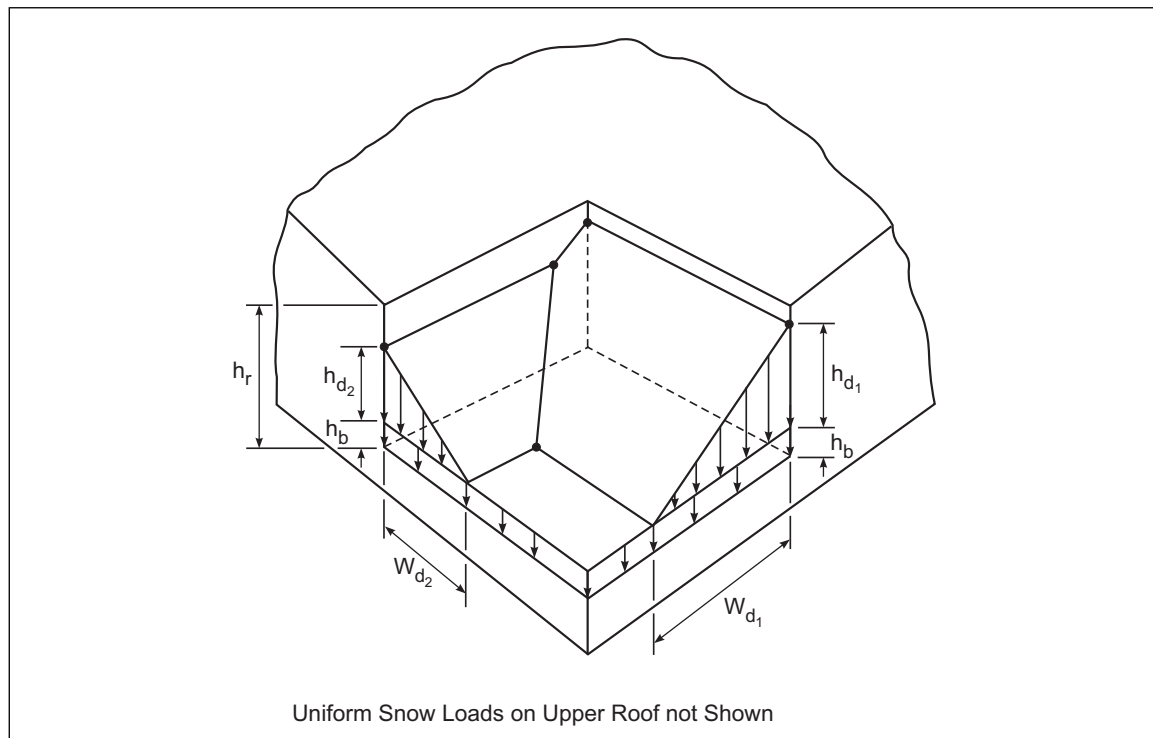
Fig. C.3.1.2-9. Snow drift intersection at lower roofs
