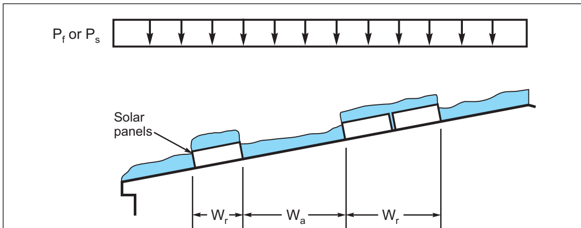
Fig. 2.5.2.3-3. Balanced snow loads on roofs with flush-mounted solar panels
