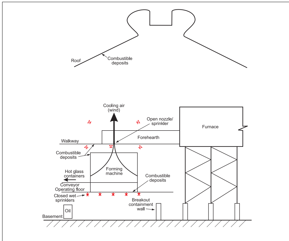
Fig. 7. Overview of fire hazards and fire protection (elevation view)
