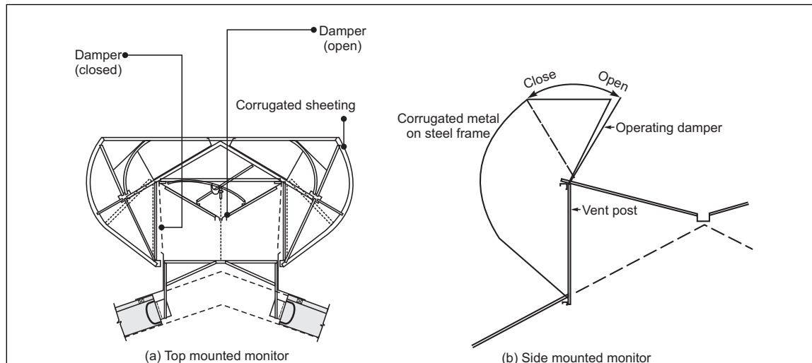
Fig. 1. Example roof monitors (cross section)
