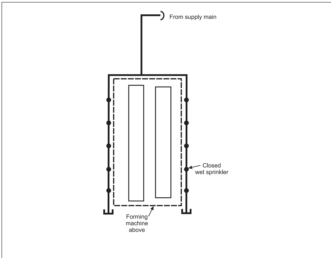
Fig. 2. Automatic sprinkler locations in basement (plan view)
