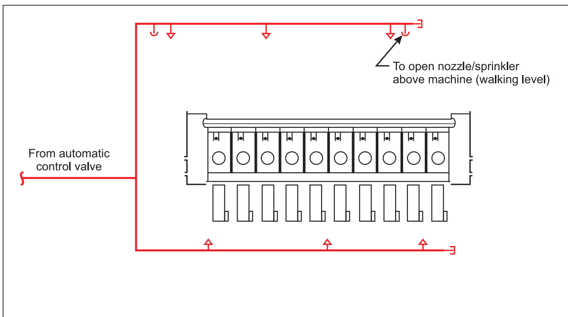
Fig. 3. Deluge sprinkler/nozzle locations at machine level (plan view)
