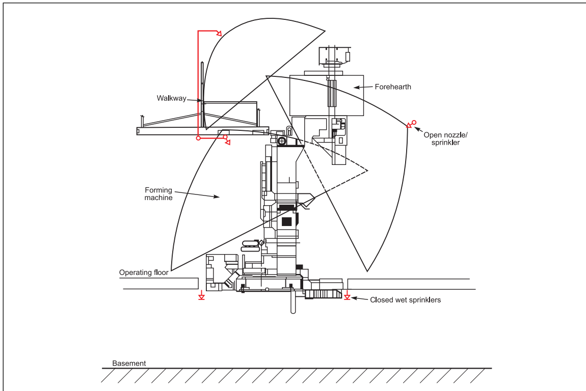
Fig. 5. Deluge sprinkler/nozzle locations around machine (elevation view 1)
