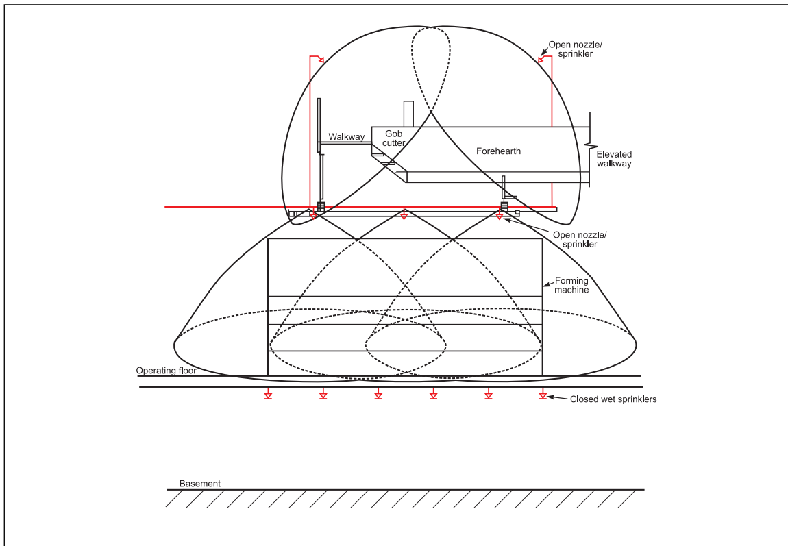
Fig. 6. Deluge sprinkler/nozzle locations around machine (elevation view 2)
