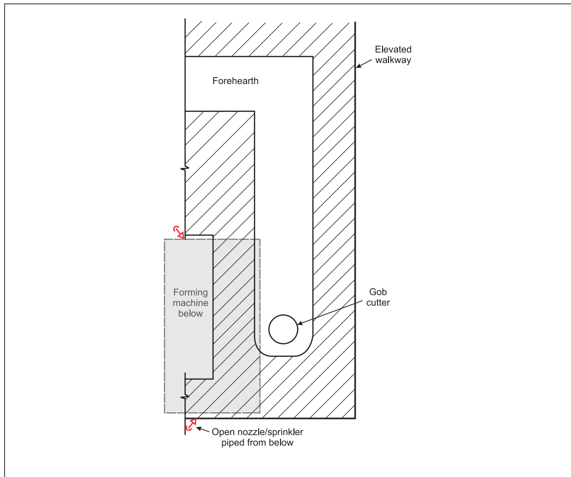
Fig. 4. Deluge sprinkler/nozzle locations above the machine (plan view)
