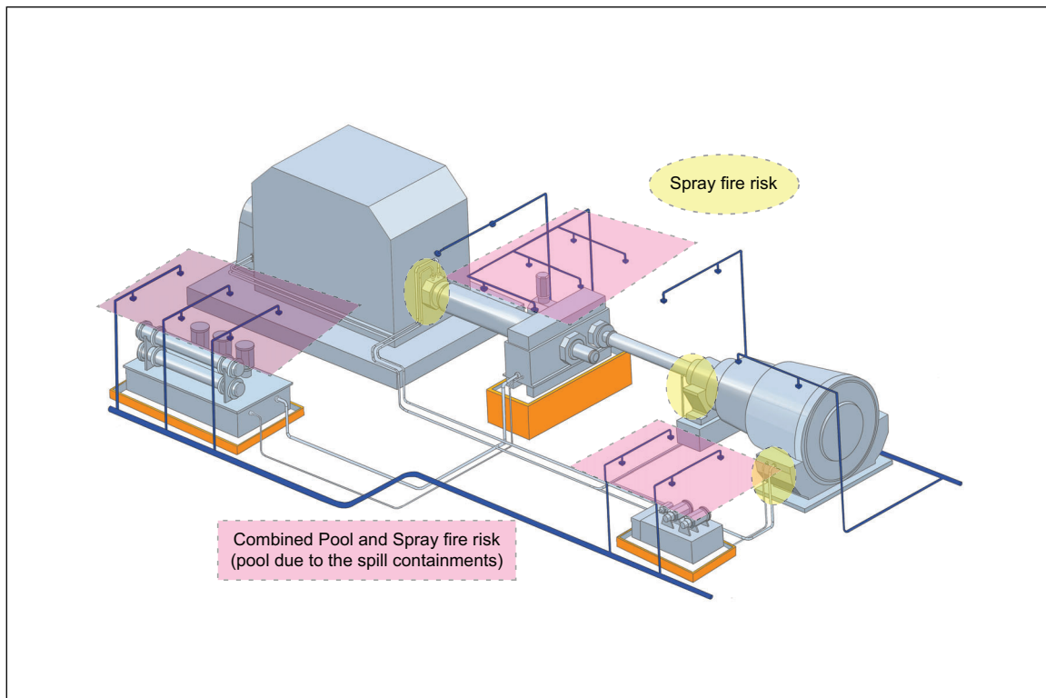
Fig. 2.4.6.2.1. Typical layout of a water mist system for local application over oil fire hazards (NOTE: Shaded areas are not solid barriers, but areas of operation.)
