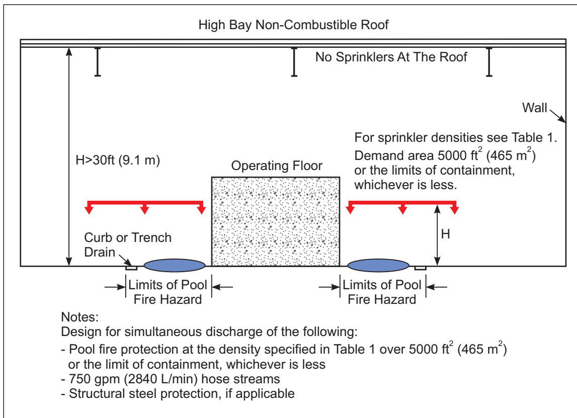
Fig. 9g. Local protection for solid pedestal designs
