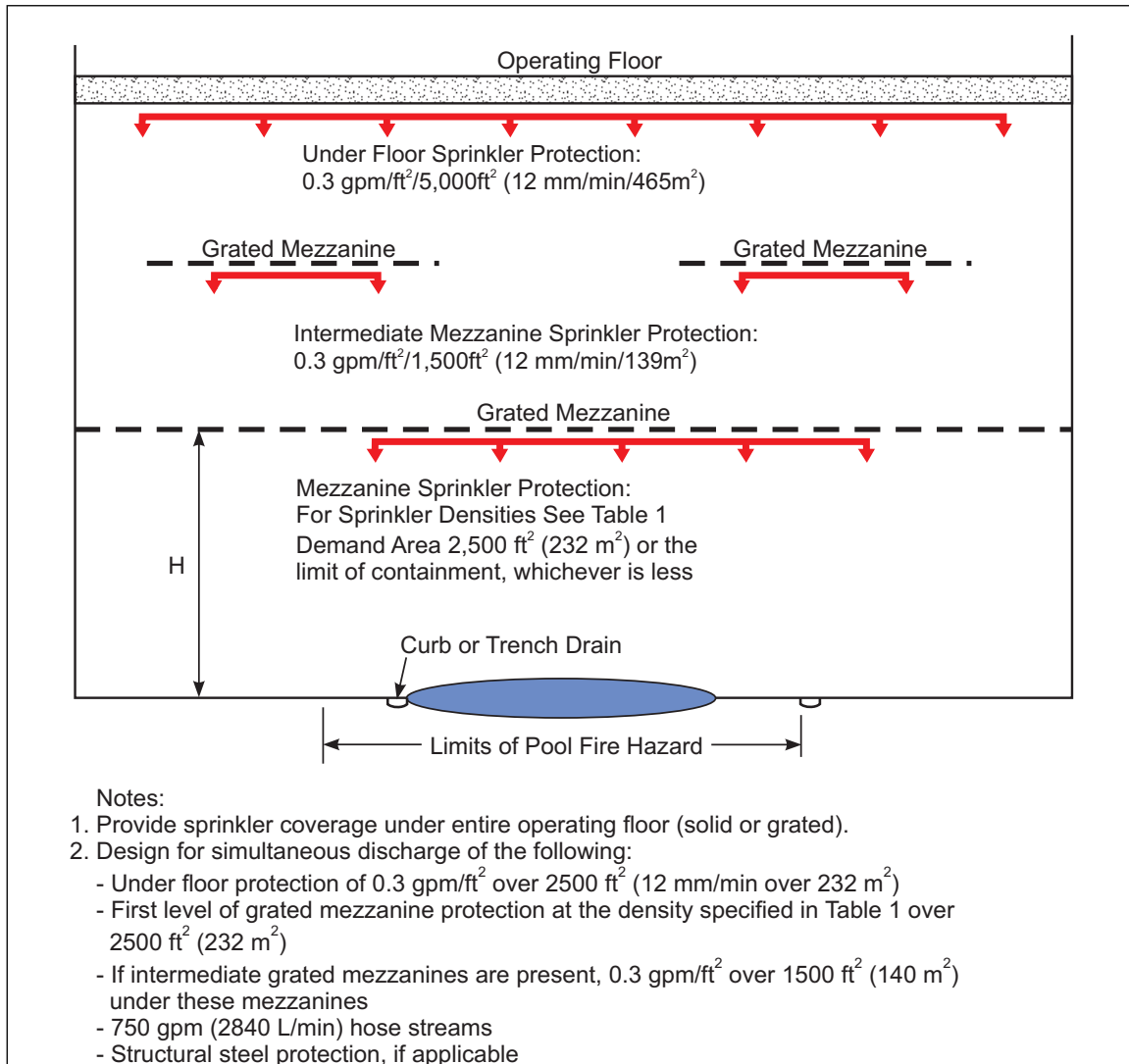
Fig. 9c. Protection for turbine buildings with solid operating floor and grated mezzanines below
