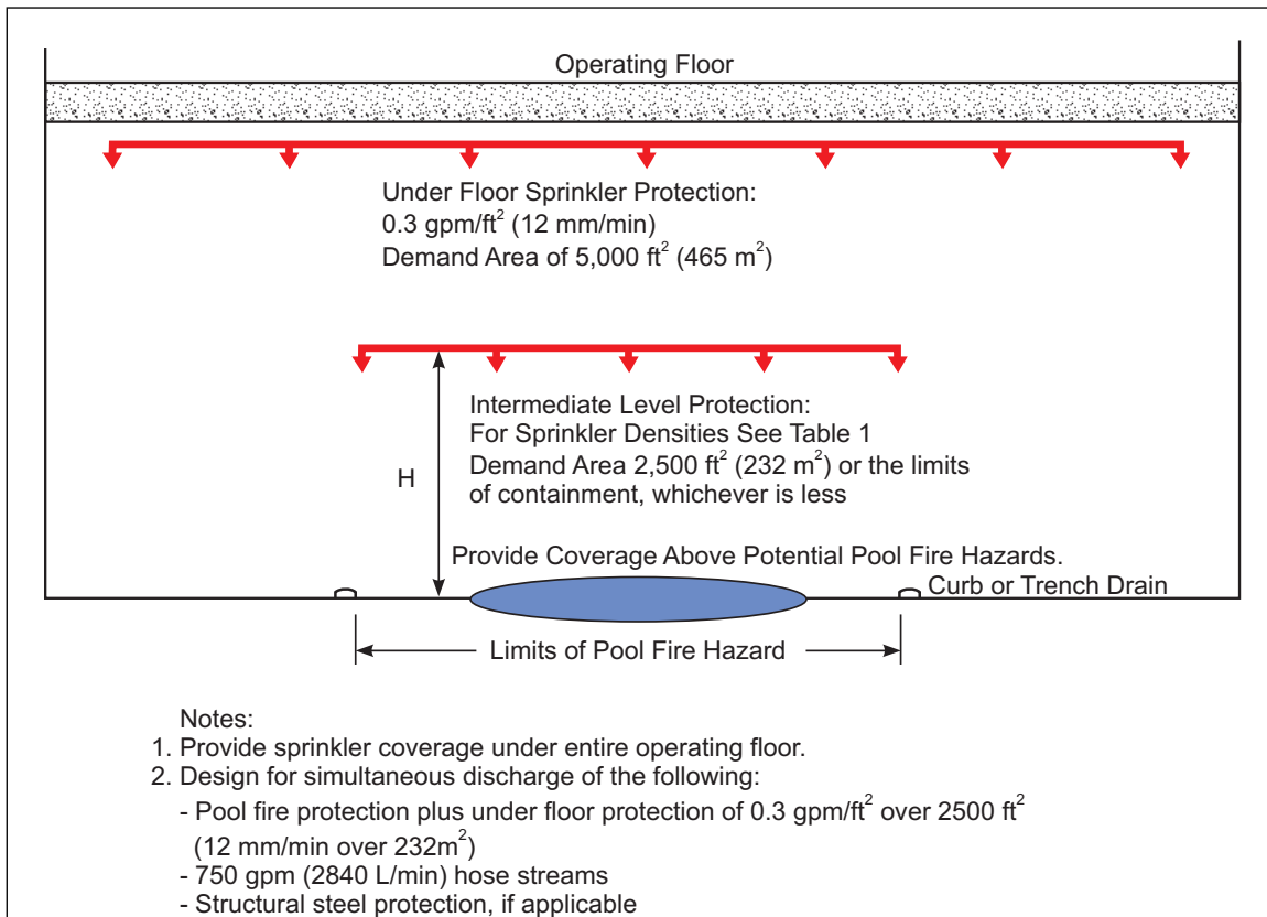
Fig. 9b. Optional protection for turbine buildings with solid operating floors higher than 30 ft (9.1 m)
