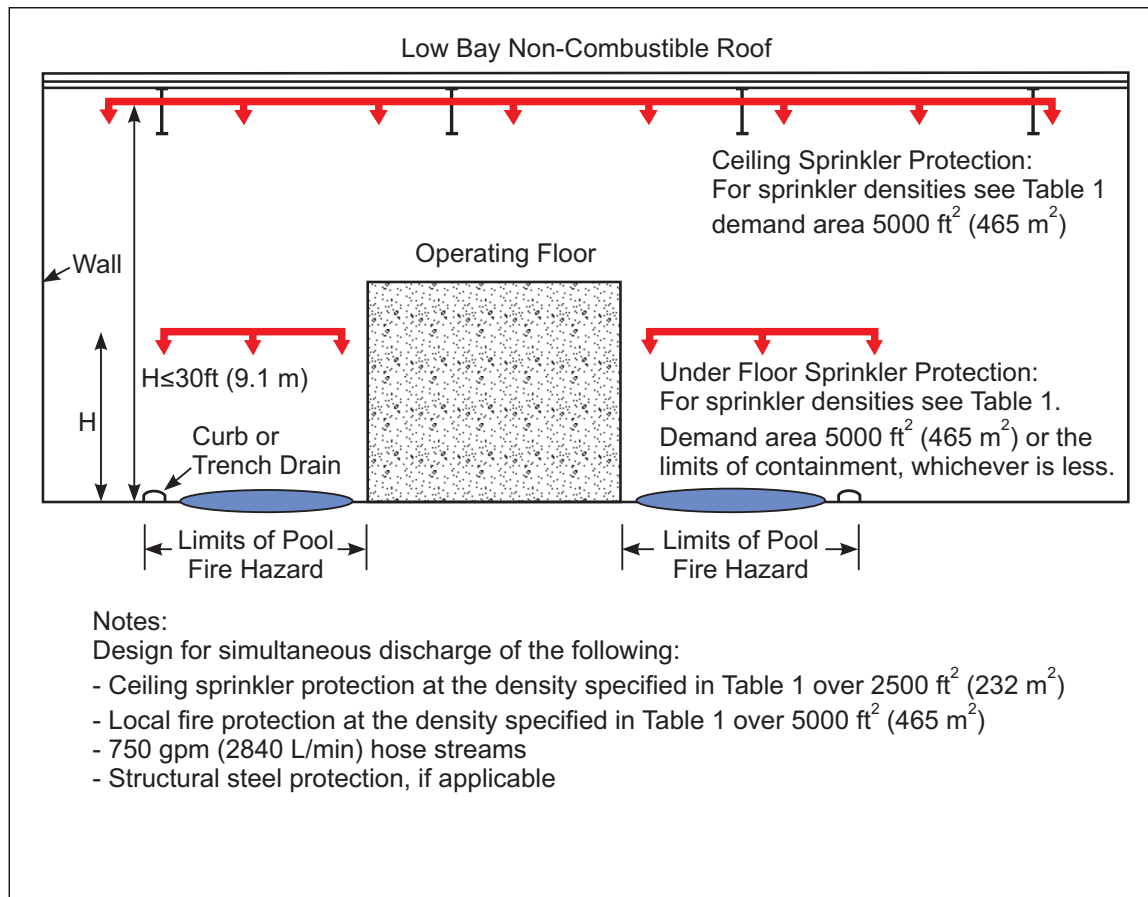
Fig. 9h. Protection for solid pedestal designs with roof height within Table 1 or less
