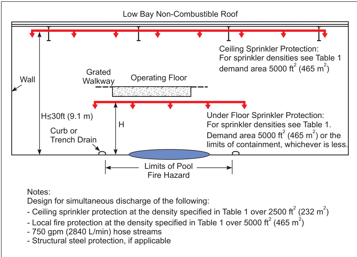
Fig. 9f. Protection for island-type turbine buildings with roof height within Table 1 or less
