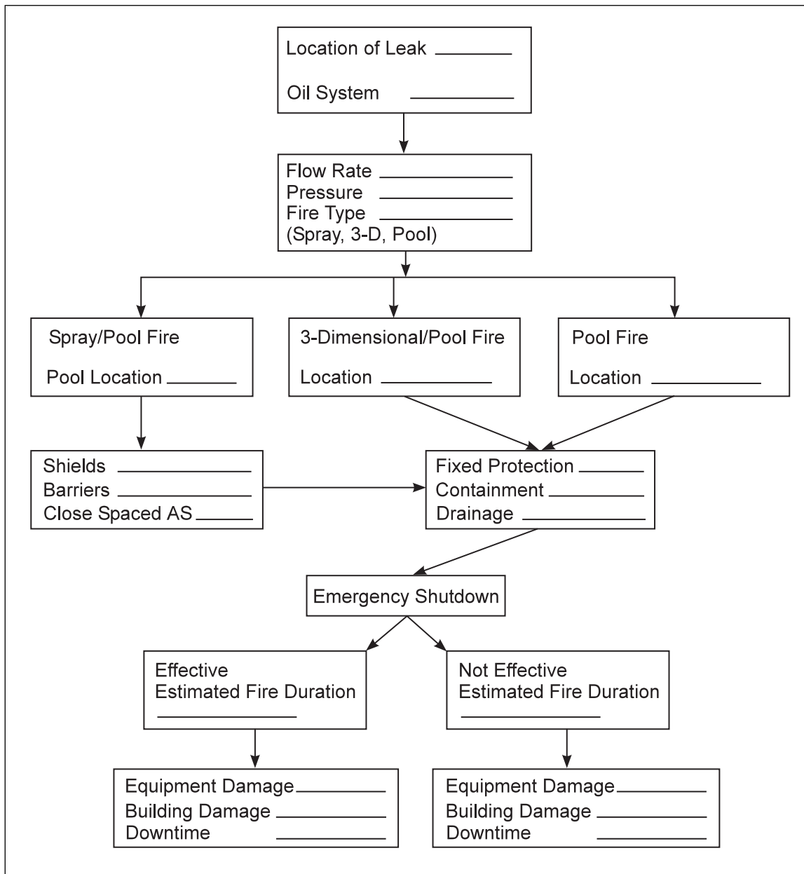
Fig. 13. Suggested outline for development of oil release and fire scenarios
