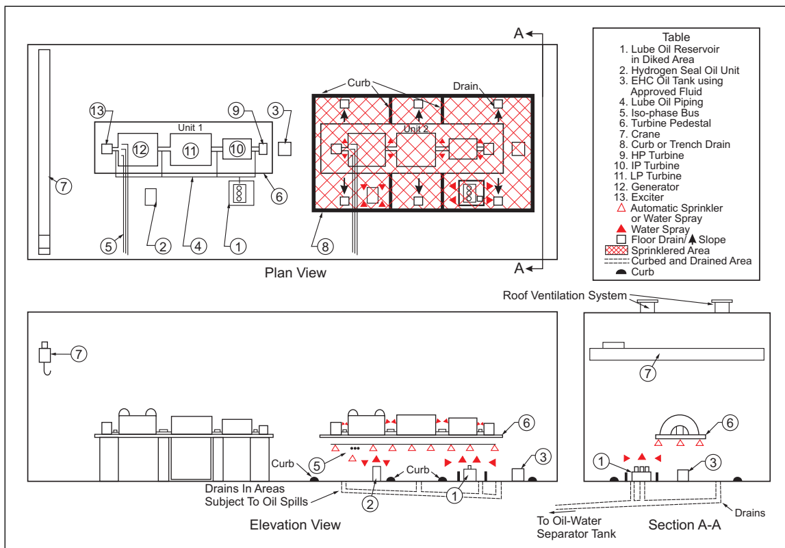
Fig. 2. Fire protection and drainage for island type turbine-generator
