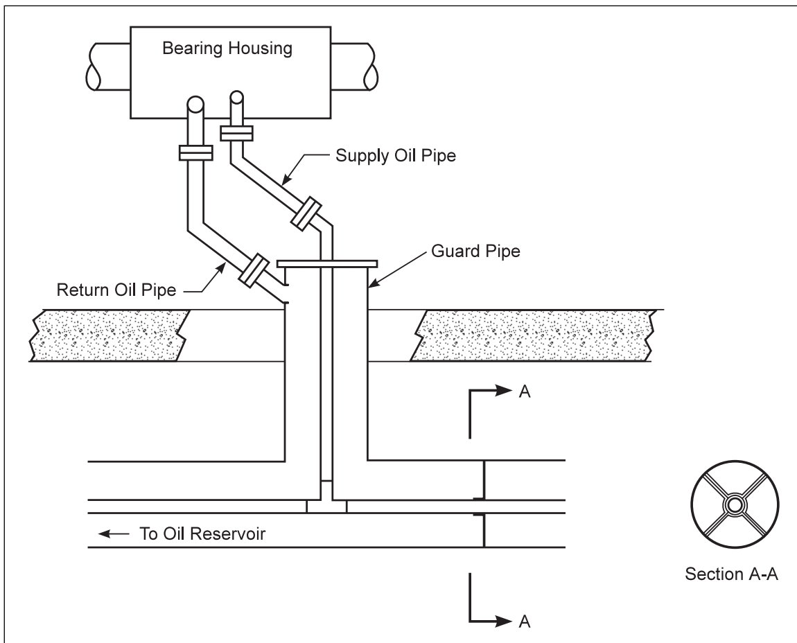
Fig. 5. Guard piping
