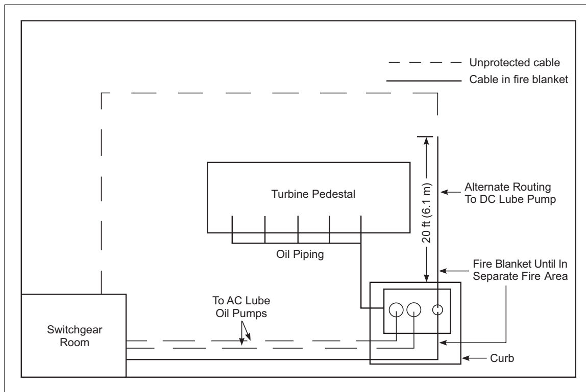
Fig. 3. Cable protection for dc lube oil pump
