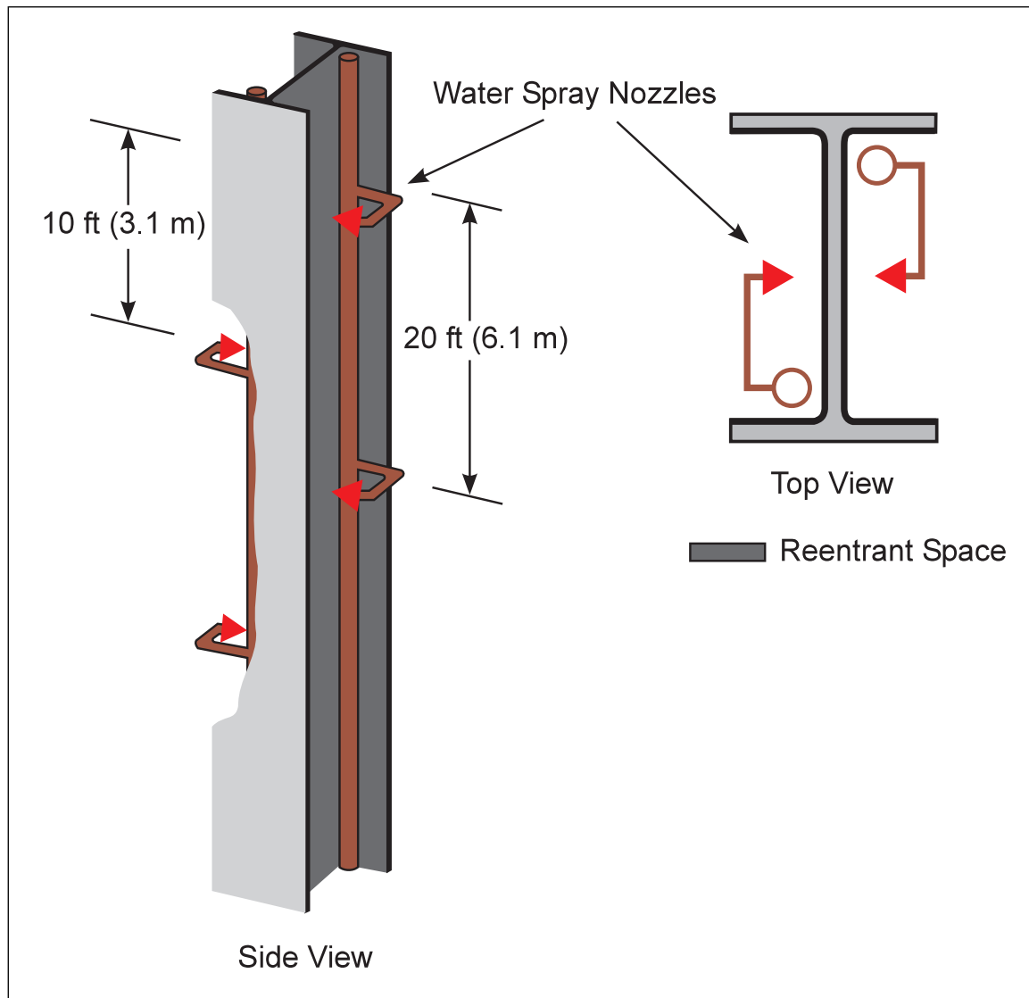
Fig. 1b. Water spray protection for steel columns
