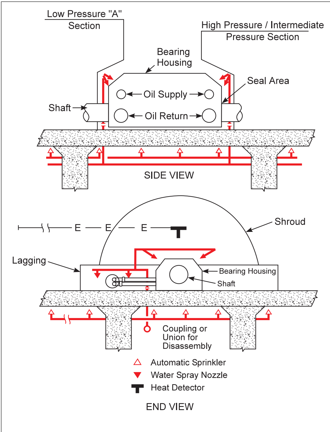
Fig. 10. Protection for bearing housing and areas under turbine skirts
