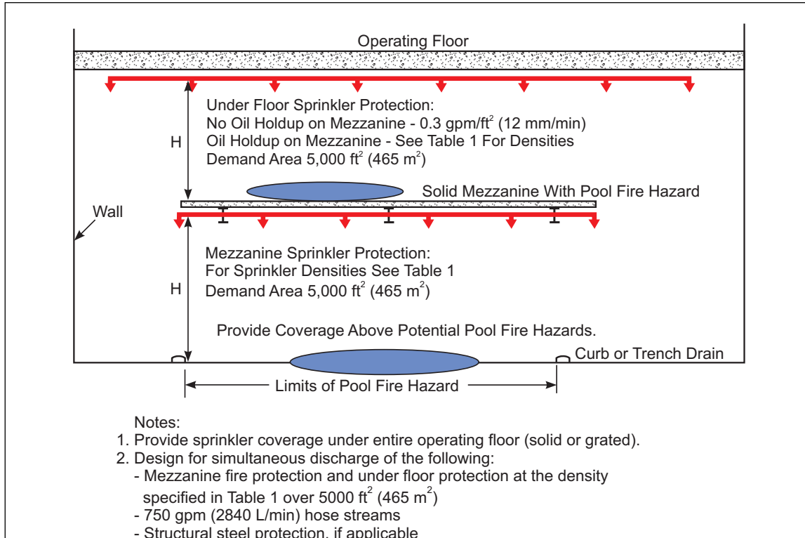
Fig. 9d. Protection for turbine buildings with solid operating floor and solid floor mezzanines
