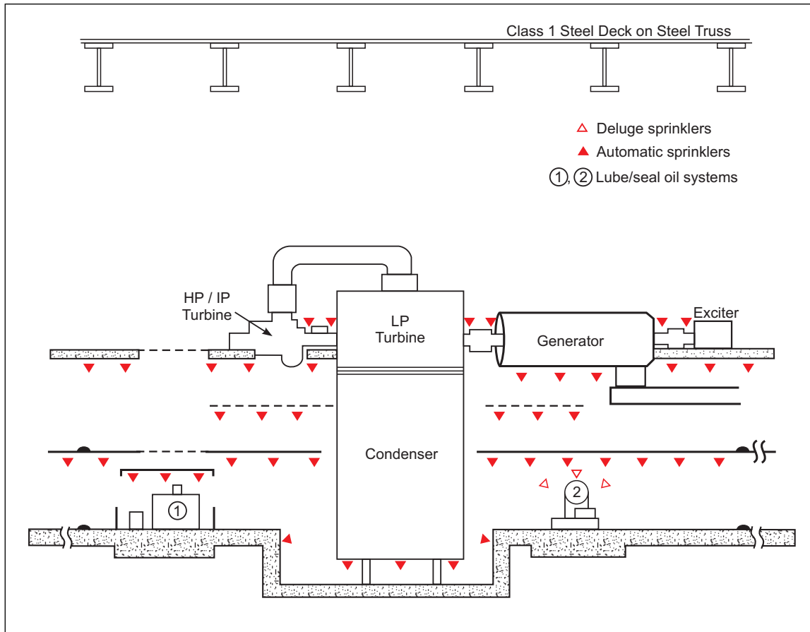
Fig. 8. Protection for medium size turbine generator with floor openings near mineral oil systems needing spray fire protection
