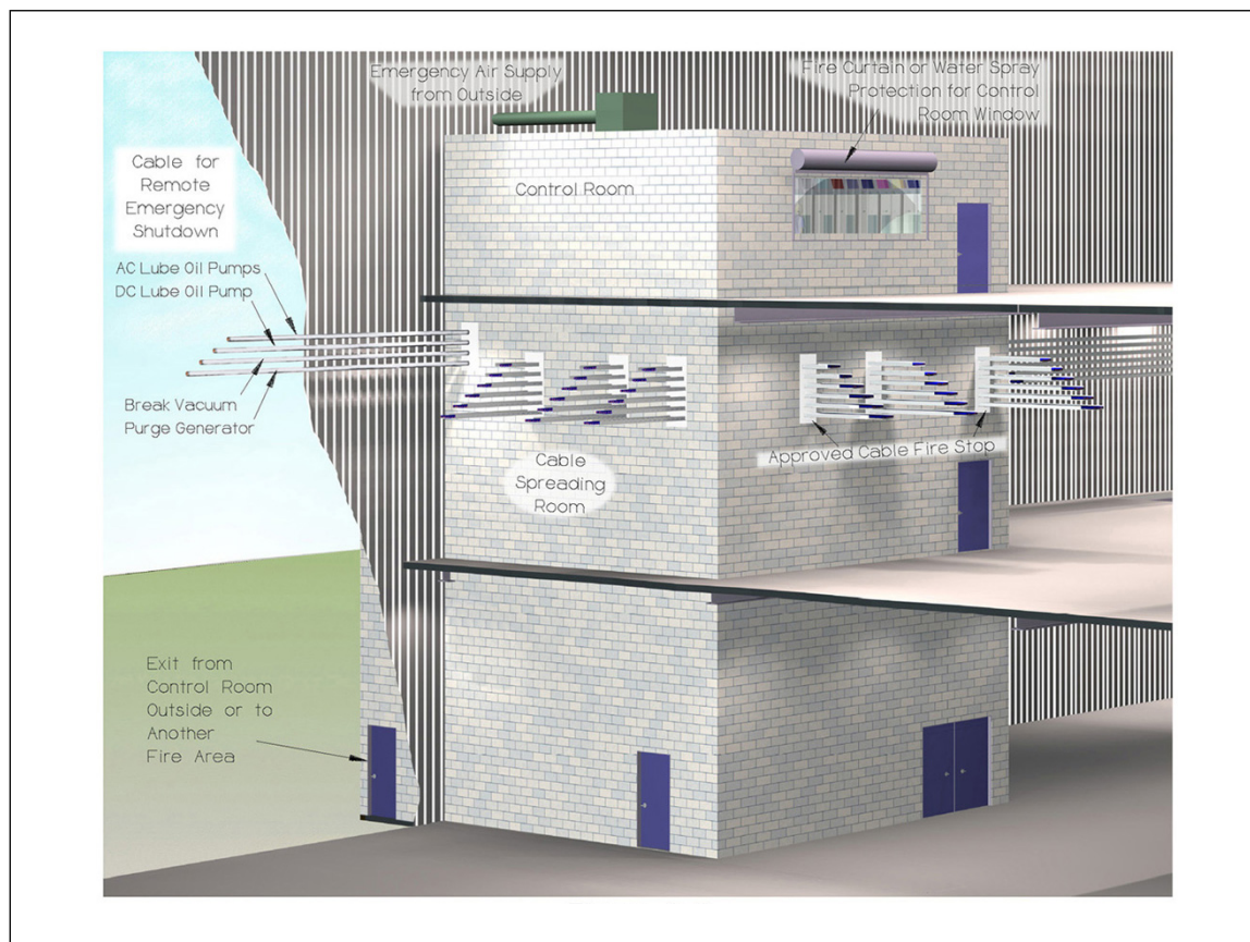
Fig. 7. Control room protection and protection of cable for remote turbine shutdown
