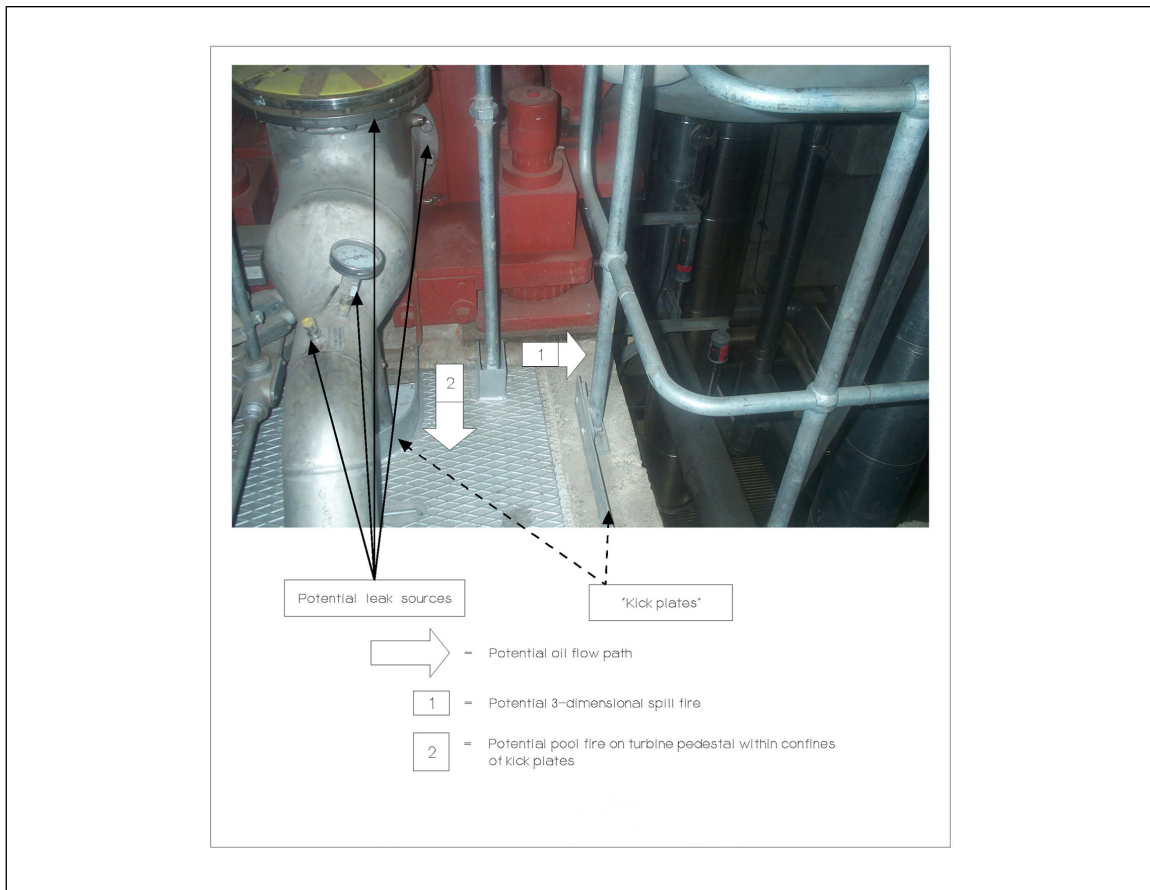
Fig. 12. Walk-down of oil system showing release and flow path
