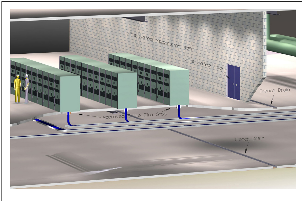
Fig. 6. Protection of electrical equipment from mineral oil fire exposure
