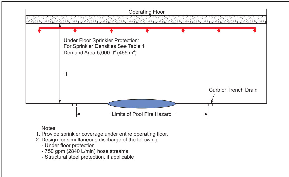
Fig. 9a. Protection for turbine buildings with solid operating floors
