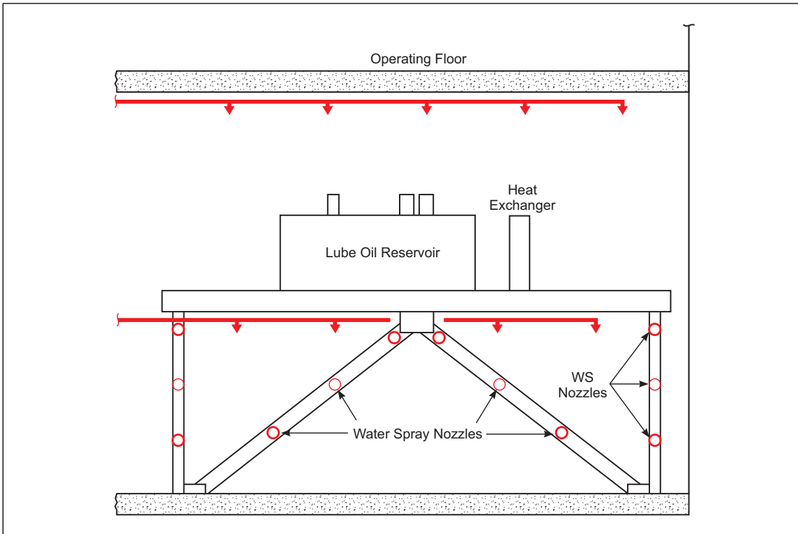
Fig. 1a. Elevated lube oil reservoir shows protection of exposed steel.
