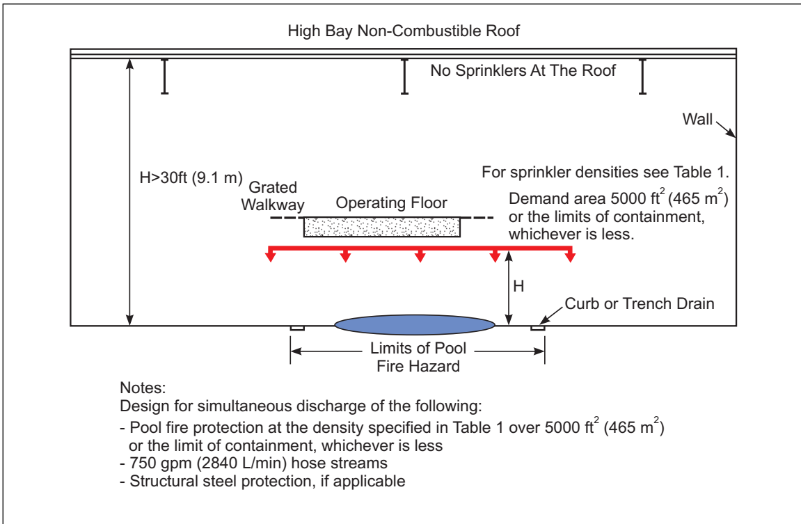
Fig. 9e. Local protection for island type turbine buildings
