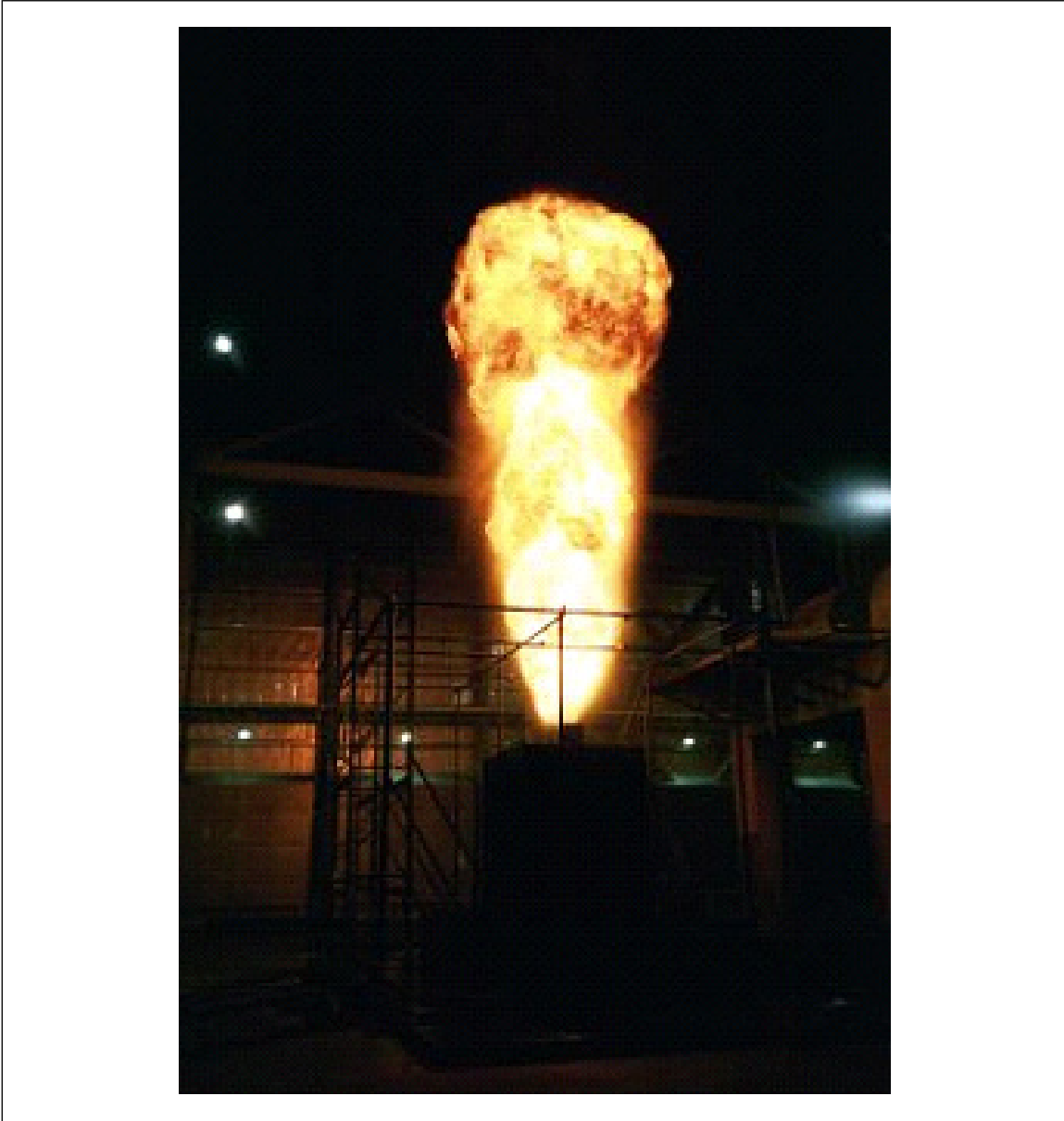
Fig. 11. Mineral oil spray fire (90 psig [6 barg]) demonstration test
