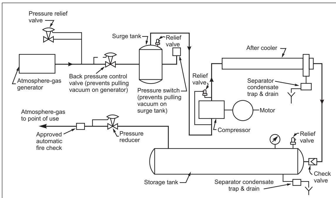
Fig. 19. Schematic piping diagram of a typical atmosphere gas-storage system.
