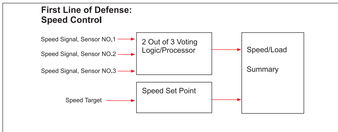
Fig. 3.2-1. Electronic speed sensing system
